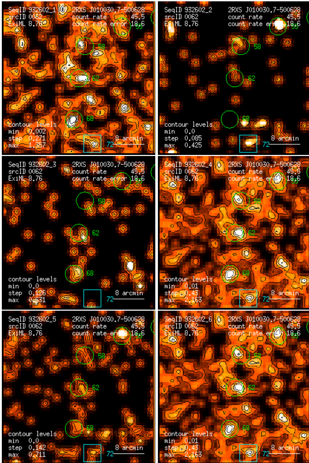
Figure 62: RASS 932602: detection 0062: band rate images, Gaussian filter: (1) PSPC channels 11 – 41, (2) 52 – 90, (3) 91 – 201, (4) 11 – 235, (5) 52 – 201, (6) 11 – 201. Broad band rates in counts/ks. Band rate contour levels in counts/ks/arcmin 2 .
