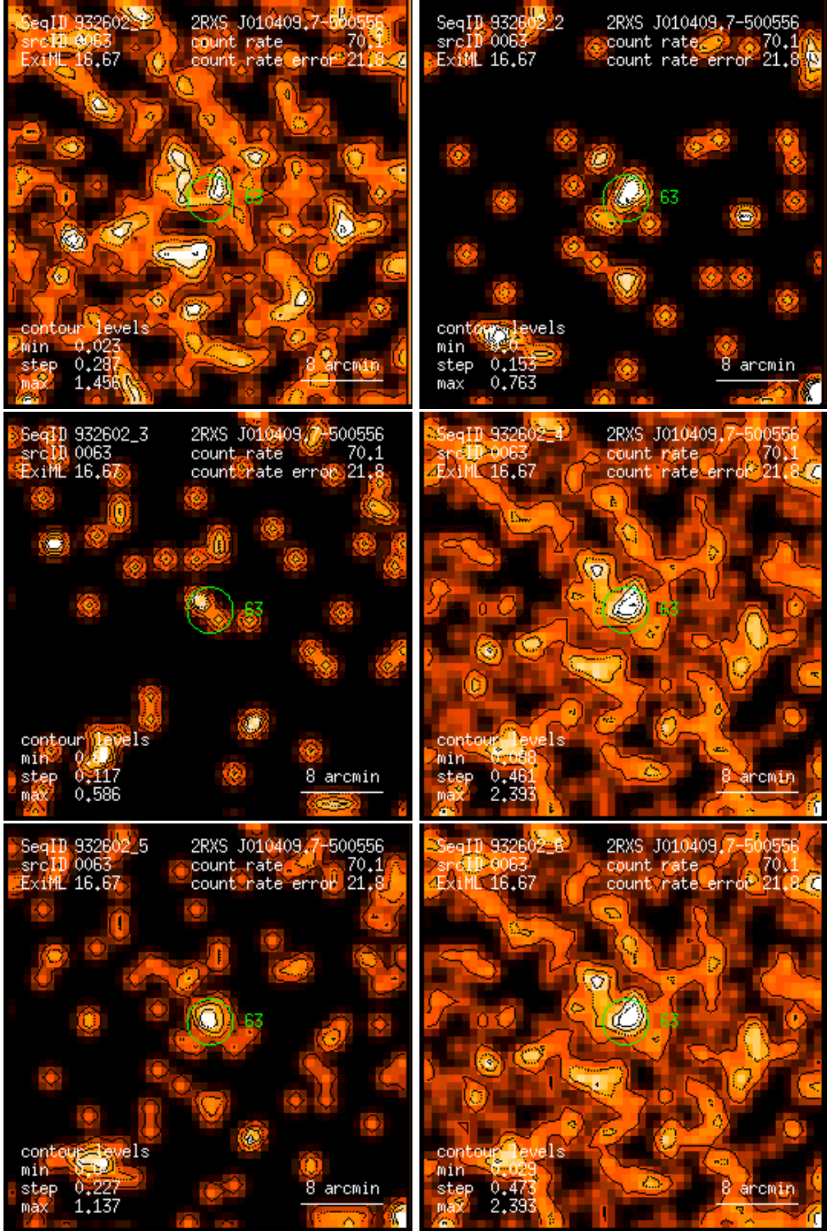
Figure 63: RASS 932602: detection 0063: band rate images, Gaussian filter: (1) PSPC channels 11 – 41, (2) 52 – 90, (3) 91 – 201, (4) 11 – 235, (5) 52 – 201, (6) 11 – 201. Broad band rates in counts/ks. Band rate contour levels in counts/ks/arcmin 2 .
