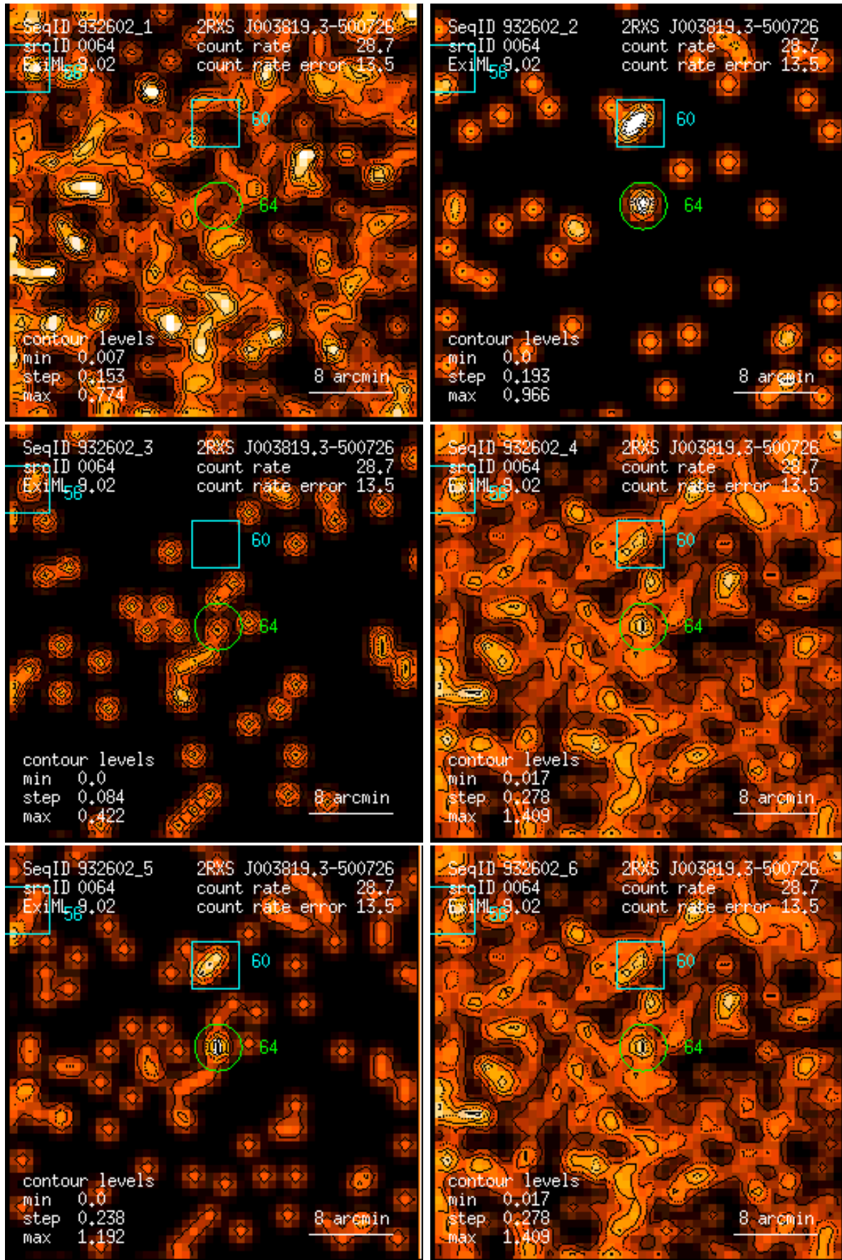
Figure 64: RASS 932602: detection 0064: band rate images, Gaussian filter: (1) PSPC channels 11 – 41, (2) 52 – 90, (3) 91 – 201, (4) 11 – 235, (5) 52 – 201, (6) 11 – 201. Broad band rates in counts/ks. Band rate contour levels in counts/ks/arcmin 2 .
