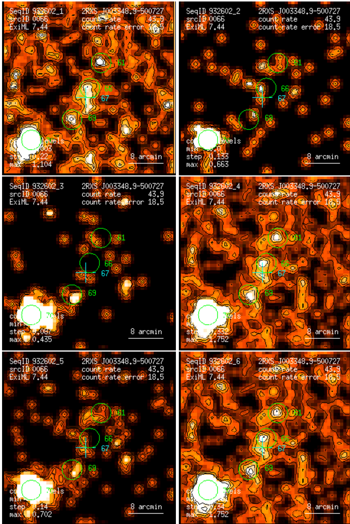
Figure 66: RASS 932602: detection 0066: band rate images, Gaussian filter: (1) PSPC channels 11 – 41, (2) 52 – 90, (3) 91 – 201, (4) 11 – 235, (5) 52 – 201, (6) 11 – 201. Broad band rates in counts/ks. Band rate contour levels in counts/ks/arcmin 2 .
