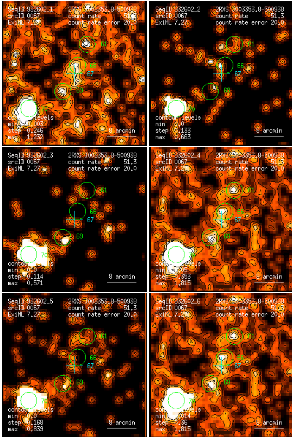
Figure 67: RASS 932602: detection 0067: band rate images, Gaussian filter: (1) PSPC channels 11 – 41, (2) 52 – 90, (3) 91 – 201, (4) 11 – 235, (5) 52 – 201, (6) 11 – 201. Broad band rates in counts/ks. Band rate contour levels in counts/ks/arcmin 2 .
