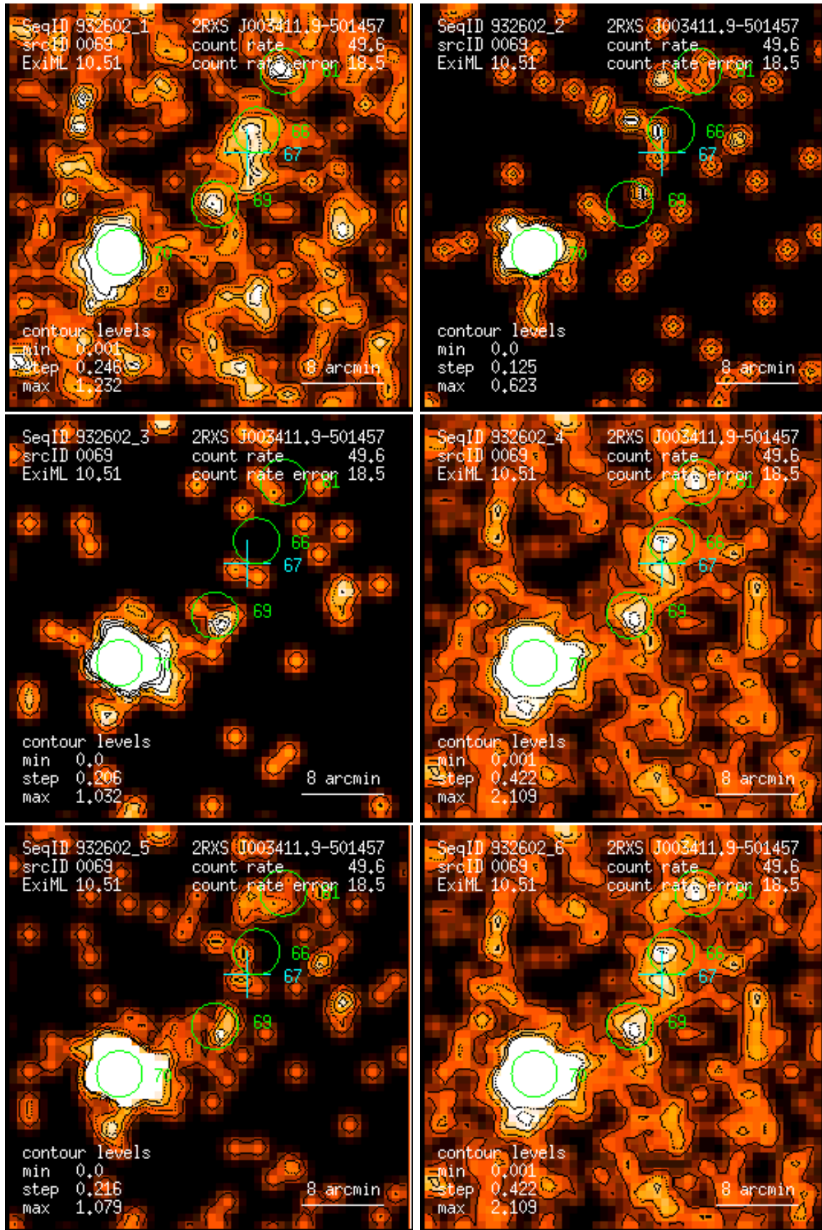
Figure 69: RASS 932602: detection 0069: band rate images, Gaussian filter: (1) PSPC channels 11 – 41, (2) 52 – 90, (3) 91 – 201, (4) 11 – 235, (5) 52 – 201, (6) 11 – 201. Broad band rates in counts/ks. Band rate contour levels in counts/ks/arcmin 2 .
