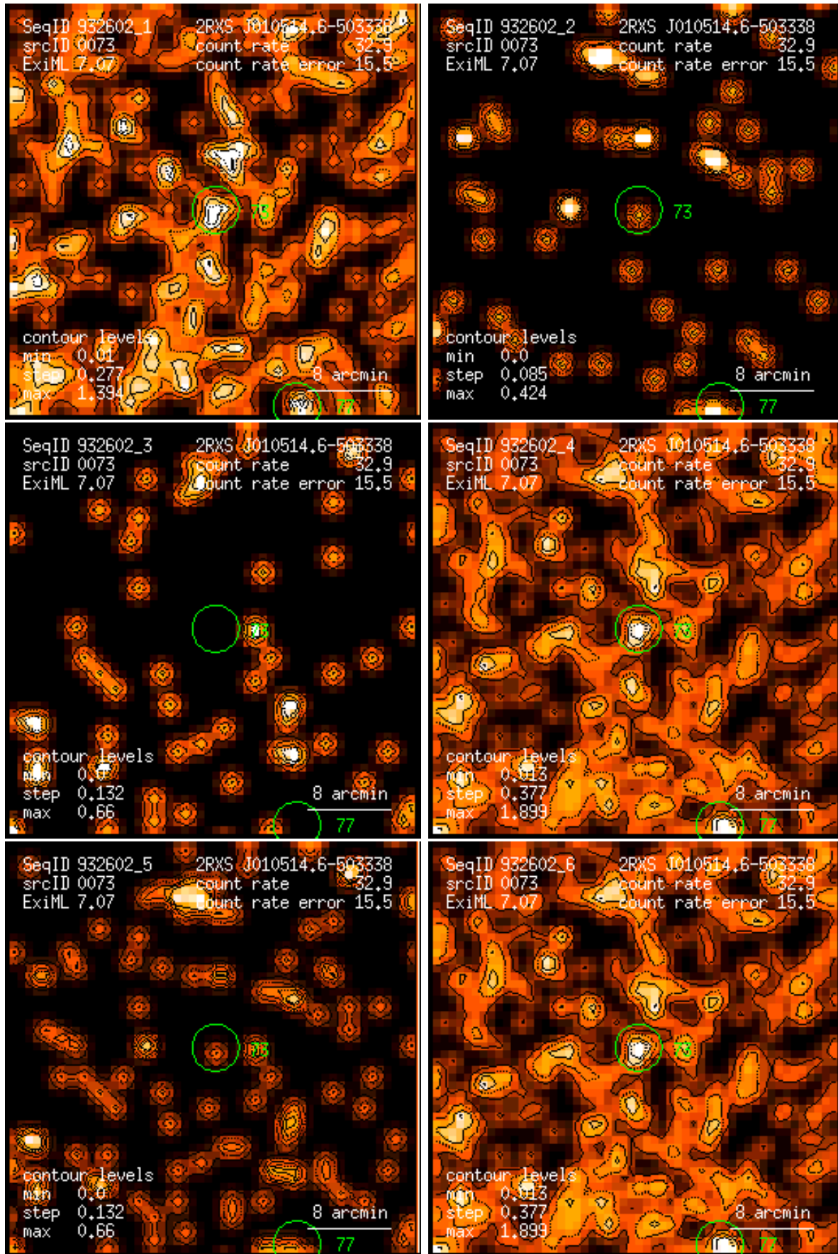
Figure 73: RASS 932602: detection 0073: band rate images, Gaussian filter: (1) PSPC channels 11 – 41, (2) 52 – 90, (3) 91 – 201, (4) 11 – 235, (5) 52 – 201, (6) 11 – 201. Broad band rates in counts/ks. Band rate contour levels in counts/ks/arcmin 2 .
