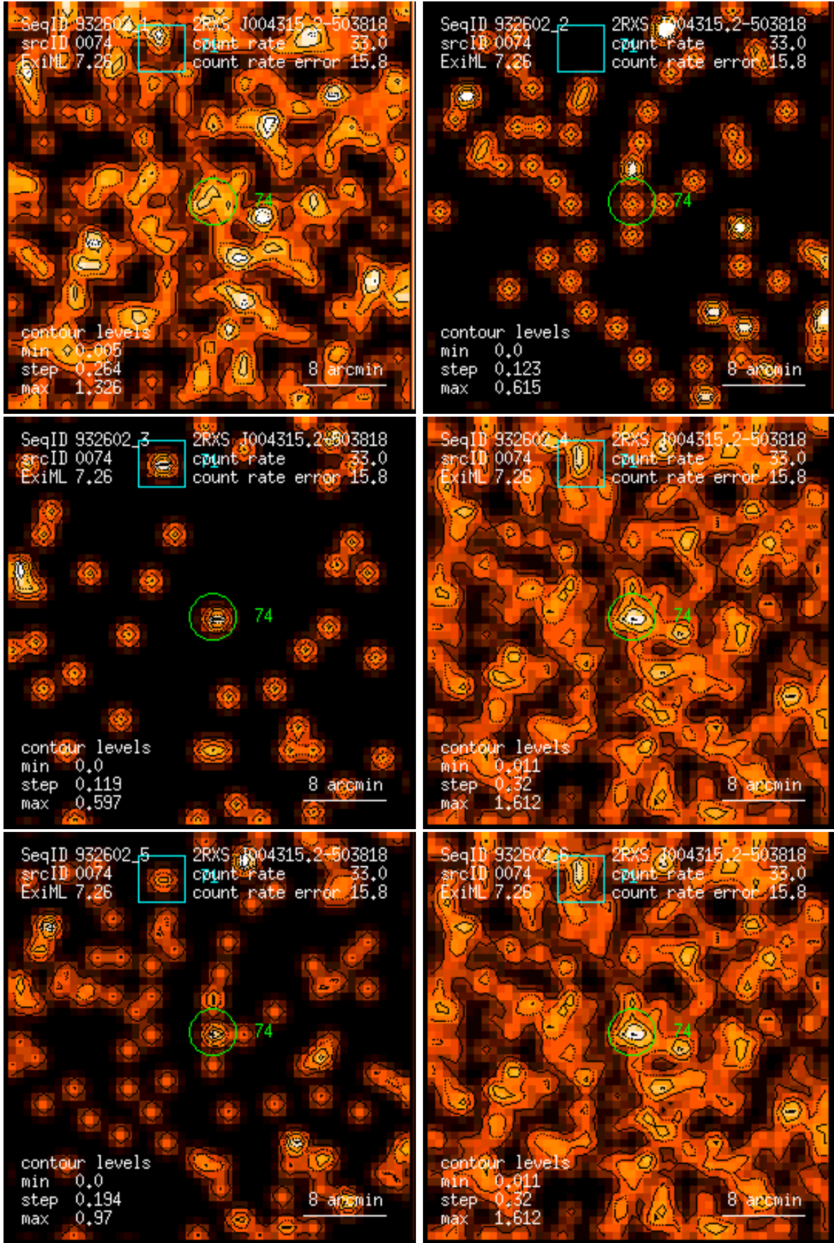
Figure 74: RASS 932602: detection 0074: band rate images, Gaussian filter: (1) PSPC channels 11 – 41, (2) 52 – 90, (3) 91 – 201, (4) 11 – 235, (5) 52 – 201, (6) 11 – 201. Broad band rates in counts/ks. Band rate contour levels in counts/ks/arcmin 2 .
