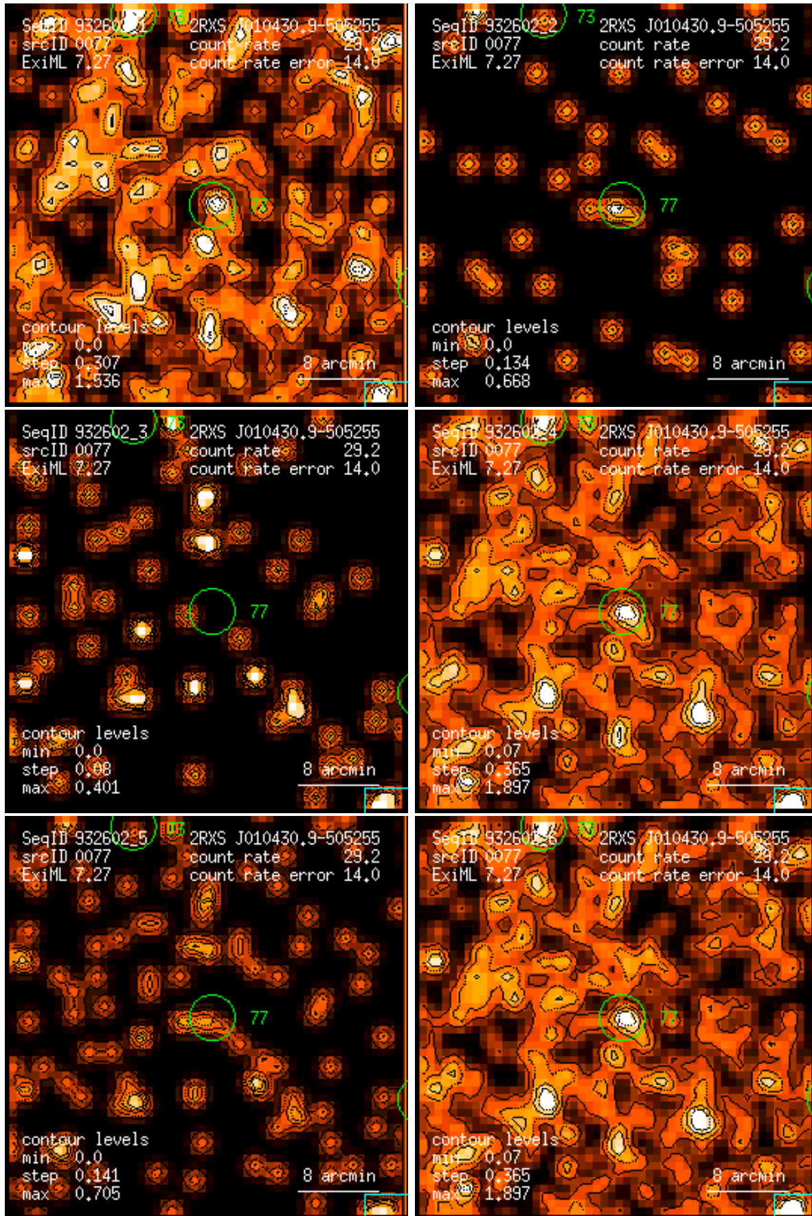
Figure 77: RASS 932602: detection 0077: band rate images, Gaussian filter: (1) PSPC channels 11 – 41, (2) 52 – 90, (3) 91 – 201, (4) 11 – 235, (5) 52 – 201, (6) 11 – 201. Broad band rates in counts/ks. Band rate contour levels in counts/ks/arcmin 2 .
