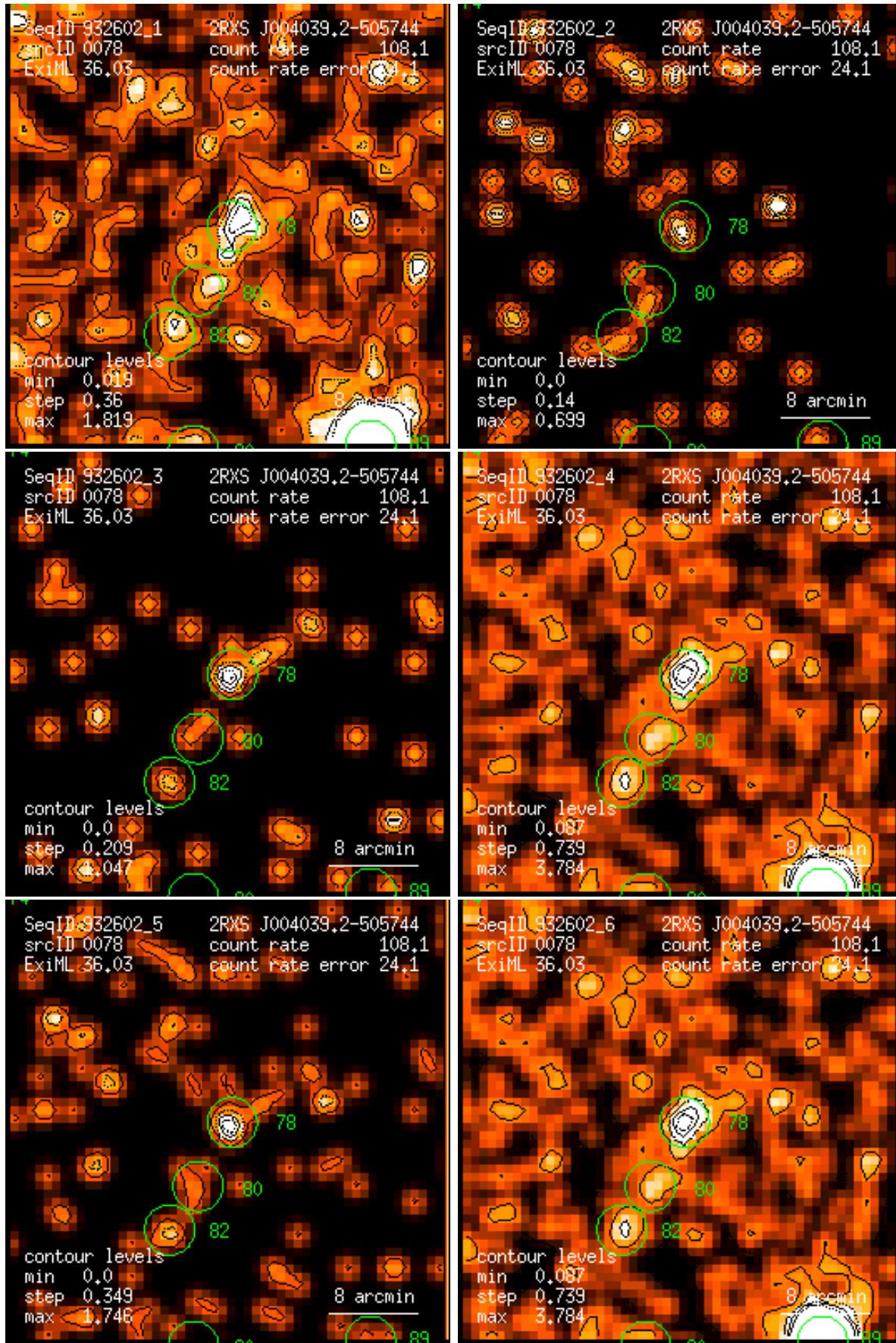
Figure 78: RASS 932602: detection 0078: band rate images, Gaussian filter: (1) PSPC channels 11 – 41, (2) 52 – 90, (3) 91 – 201, (4) 11 – 235, (5) 52 – 201, (6) 11 – 201. Broad band rates in counts/ks. Band rate contour levels in counts/ks/arcmin 2 .
