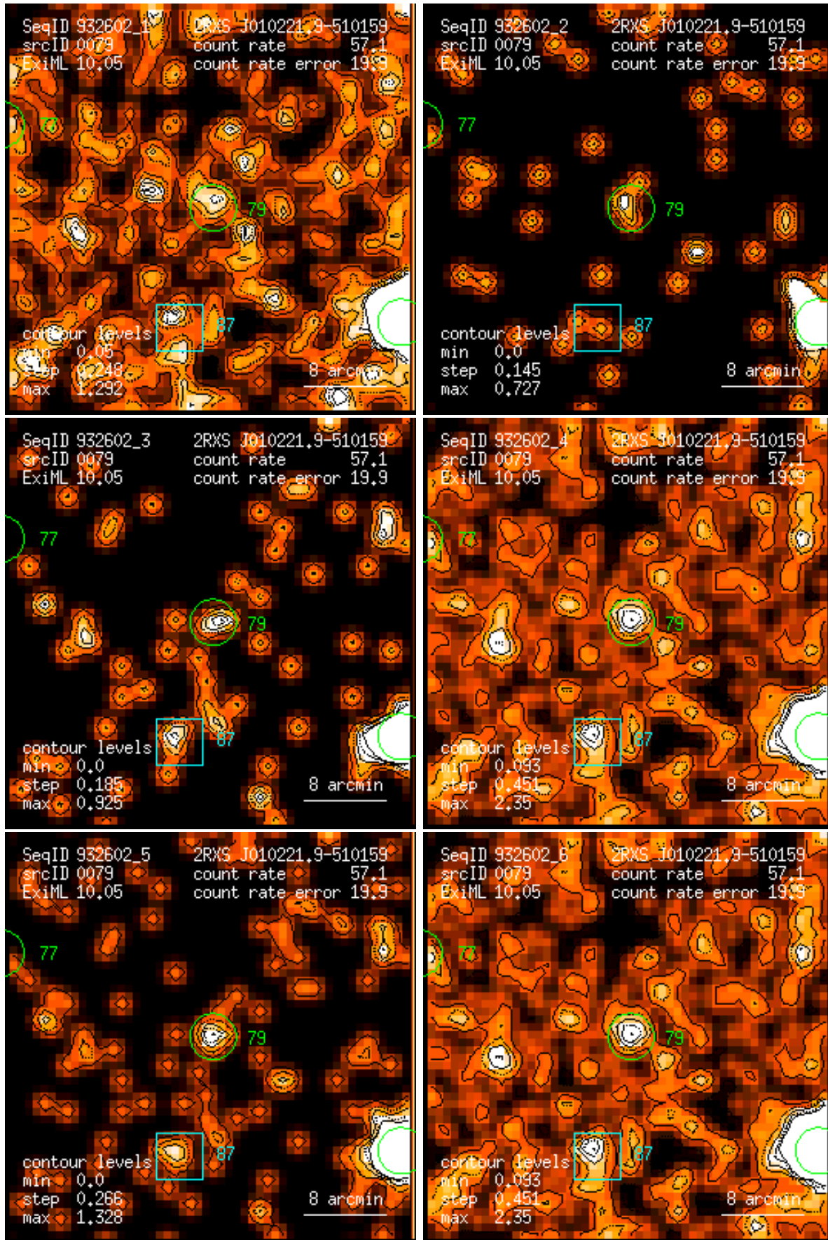
Figure 79: RASS 932602: detection 0079: band rate images, Gaussian filter: (1) PSPC channels 11 – 41, (2) 52 – 90, (3) 91 – 201, (4) 11 – 235, (5) 52 – 201, (6) 11 – 201. Broad band rates in counts/ks. Band rate contour levels in counts/ks/arcmin 2 .
