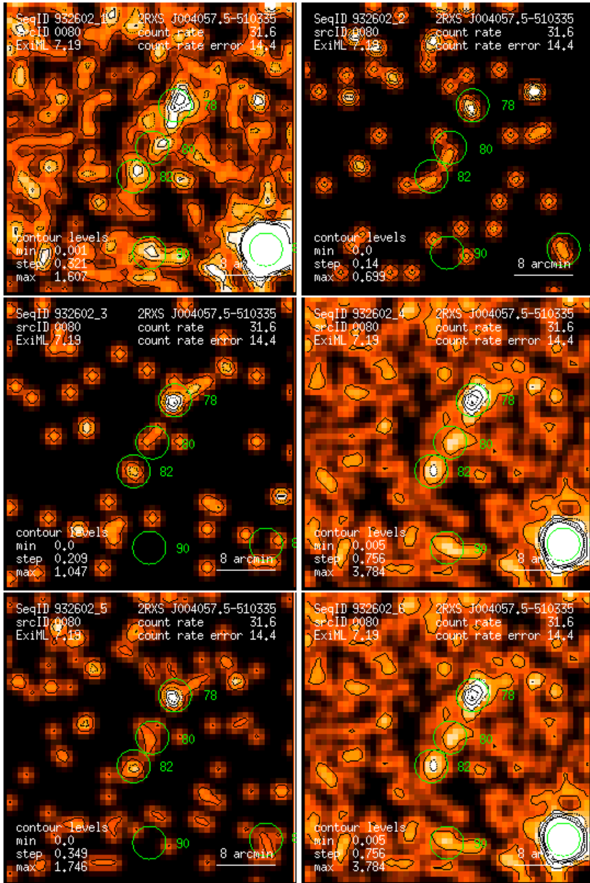
Figure 80: RASS 932602: detection 0080: band rate images, Gaussian filter: (1) PSPC channels 11 – 41, (2) 52 – 90, (3) 91 – 201, (4) 11 – 235, (5) 52 – 201, (6) 11 – 201. Broad band rates in counts/ks. Band rate contour levels in counts/ks/arcmin 2 .
