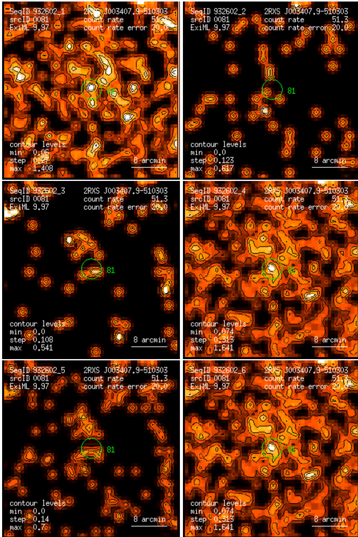
Figure 81: RASS 932602: detection 0081: band rate images, Gaussian filter: (1) PSPC channels 11 – 41, (2) 52 – 90, (3) 91 – 201, (4) 11 – 235, (5) 52 – 201, (6) 11 – 201. Broad band rates in counts/ks. Band rate contour levels in counts/ks/arcmin 2 .
