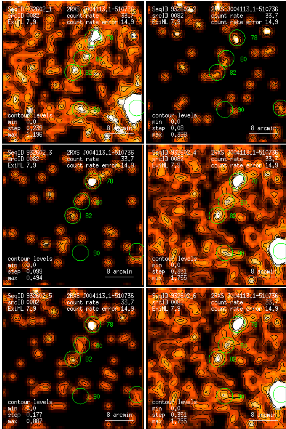
Figure 82: RASS 932602: detection 0082: band rate images, Gaussian filter: (1) PSPC channels 11 – 41, (2) 52 – 90, (3) 91 – 201, (4) 11 – 235, (5) 52 – 201, (6) 11 – 201. Broad band rates in counts/ks. Band rate contour levels in counts/ks/arcmin 2 .
