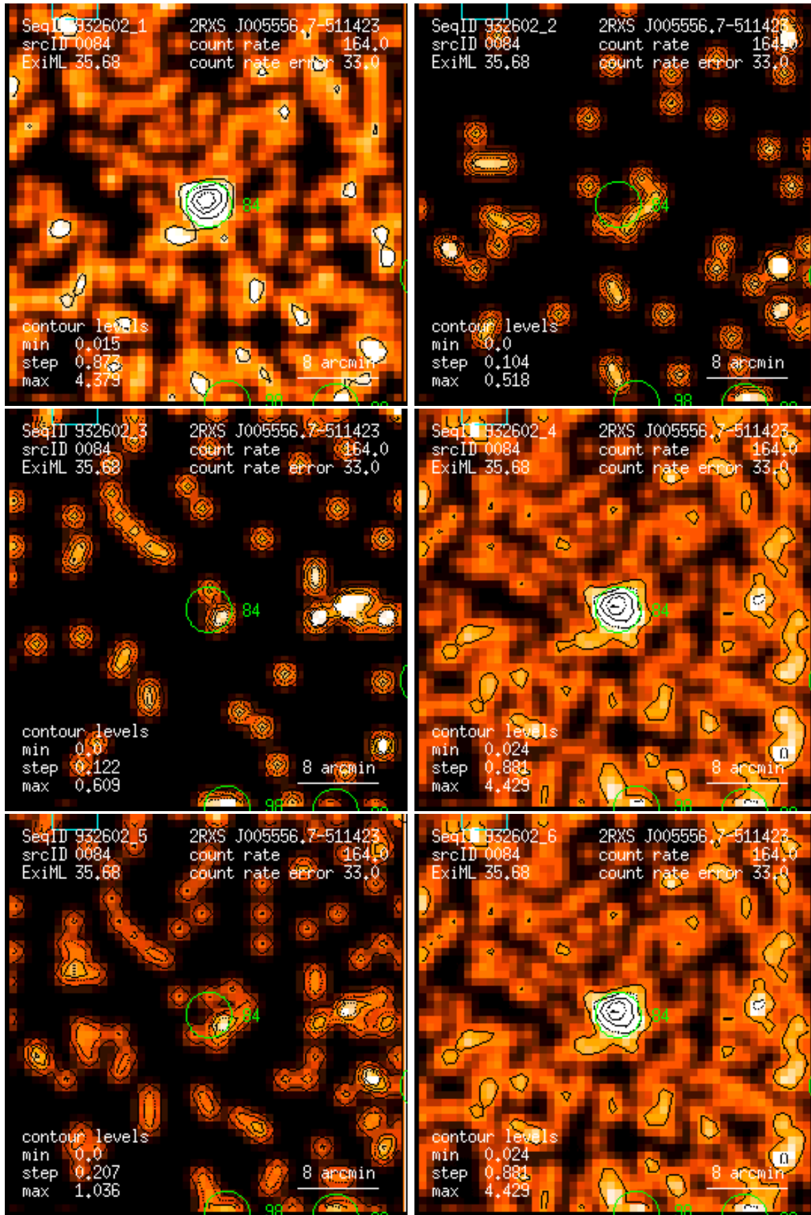
Figure 84: RASS 932602: detection 0084: band rate images, Gaussian filter: (1) PSPC channels 11 – 41, (2) 52 – 90, (3) 91 – 201, (4) 11 – 235, (5) 52 – 201, (6) 11 – 201. Broad band rates in counts/ks. Band rate contour levels in counts/ks/arcmin 2 .
