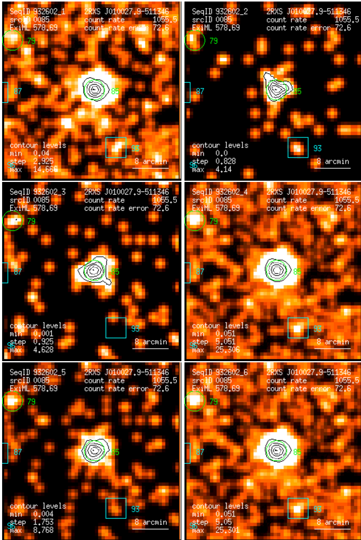
Figure 85: RASS 932602: detection 0085: band rate images, Gaussian filter: (1) PSPC channels 11 – 41, (2) 52 – 90, (3) 91 – 201, (4) 11 – 235, (5) 52 – 201, (6) 11 – 201. Broad band rates in counts/ks. Band rate contour levels in counts/ks/arcmin 2 .
