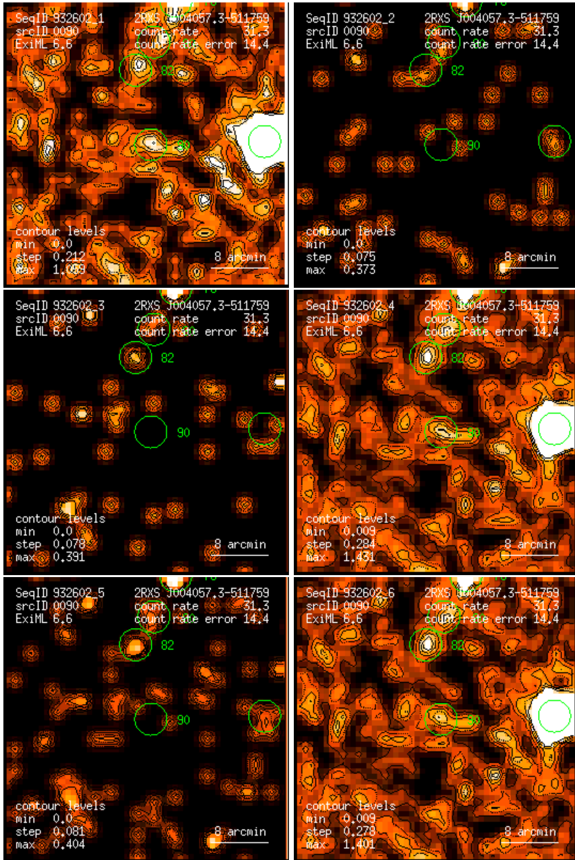
Figure 90: RASS 932602: detection 0090: band rate images, Gaussian filter: (1) PSPC channels 11 – 41, (2) 52 – 90, (3) 91 – 201, (4) 11 – 235, (5) 52 – 201, (6) 11 – 201. Broad band rates in counts/ks. Band rate contour levels in counts/ks/arcmin 2 .
