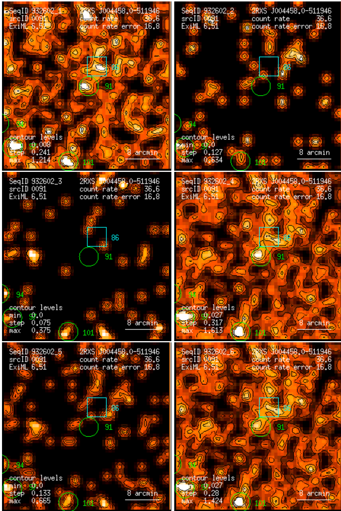
Figure 91: RASS 932602: detection 0091: band rate images, Gaussian filter: (1) PSPC channels 11 – 41, (2) 52 – 90, (3) 91 – 201, (4) 11 – 235, (5) 52 – 201, (6) 11 – 201. Broad band rates in counts/ks. Band rate contour levels in counts/ks/arcmin 2 .
