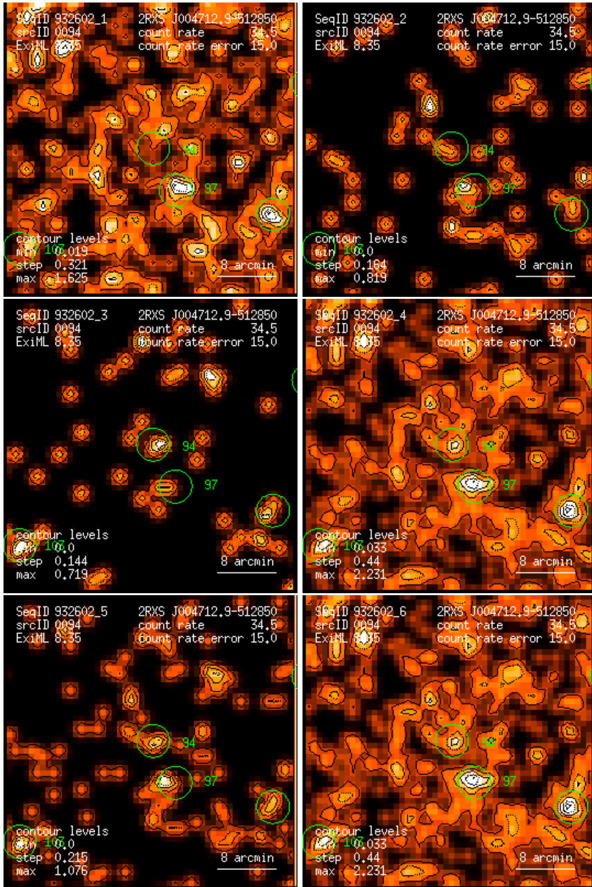
Figure 94: RASS 932602: detection 0094: band rate images, Gaussian filter: (1) PSPC channels 11 – 41, (2) 52 – 90, (3) 91 – 201, (4) 11 – 235, (5) 52 – 201, (6) 11 – 201. Broad band rates in counts/ks. Band rate contour levels in counts/ks/arcmin 2 .
