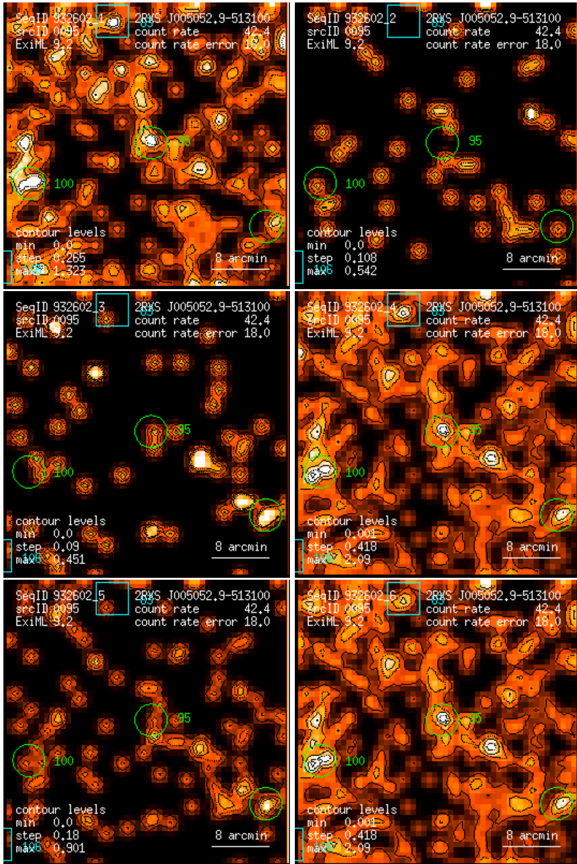
Figure 95: RASS 932602: detection 0095: band rate images, Gaussian filter: (1) PSPC channels 11 – 41, (2) 52 – 90, (3) 91 – 201, (4) 11 – 235, (5) 52 – 201, (6) 11 – 201. Broad band rates in counts/ks. Band rate contour levels in counts/ks/arcmin 2 .
