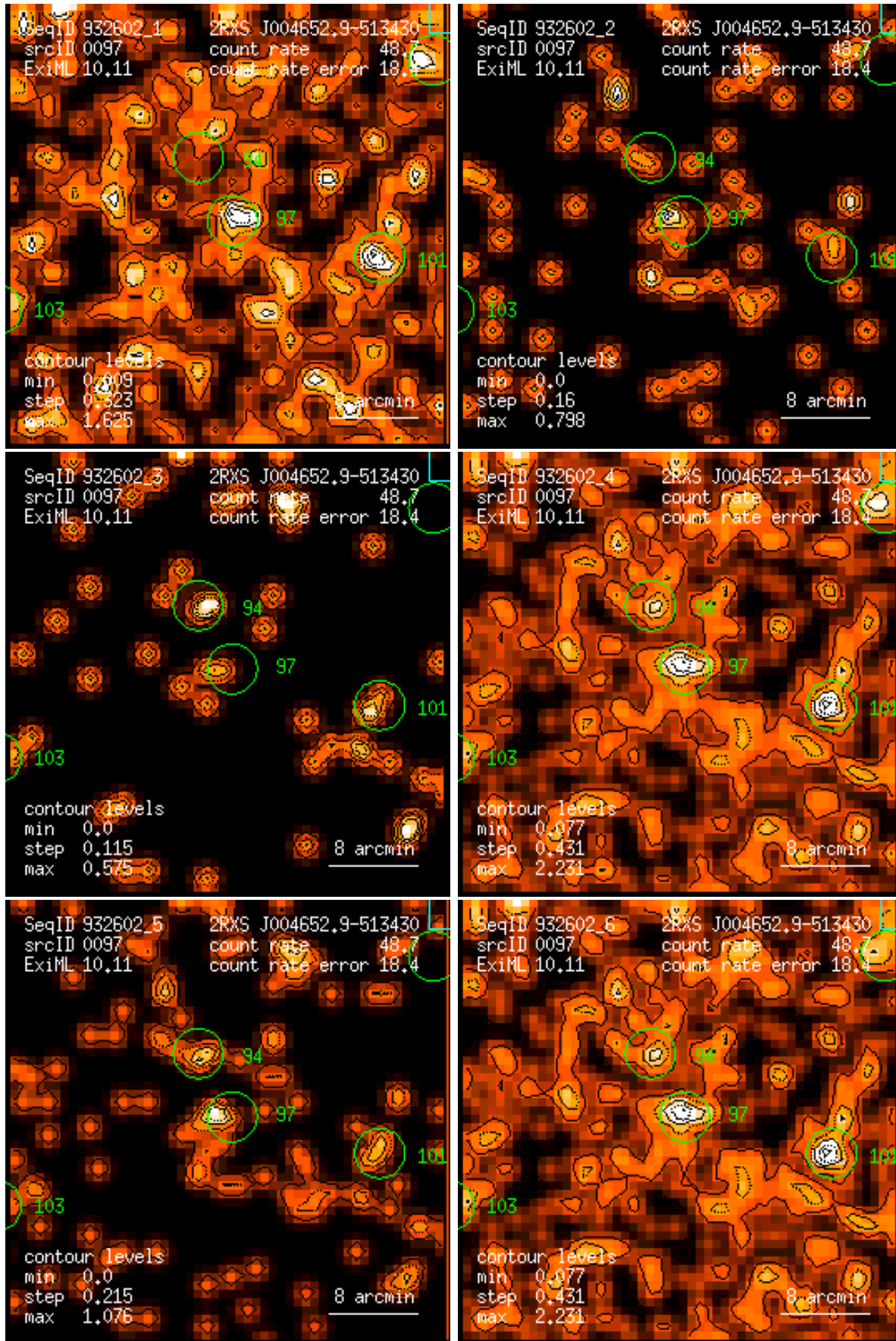
Figure 97: RASS 932602: detection 0097: band rate images, Gaussian filter: (1) PSPC channels 11 – 41, (2) 52 – 90, (3) 91 – 201, (4) 11 – 235, (5) 52 – 201, (6) 11 – 201. Broad band rates in counts/ks. Band rate contour levels in counts/ks/arcmin 2 .
