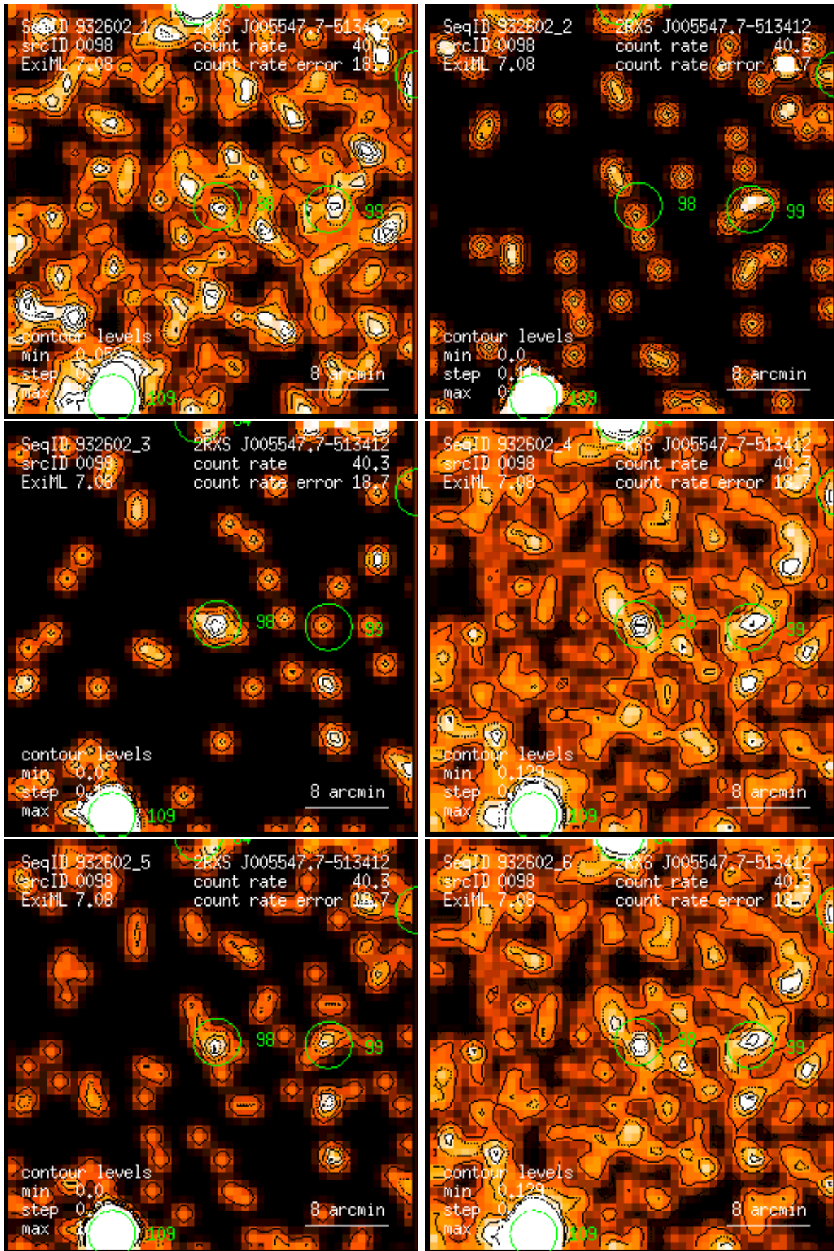
Figure 98: RASS 932602: detection 0098: band rate images, Gaussian filter: (1) PSPC channels 11 – 41, (2) 52 – 90, (3) 91 – 201, (4) 11 – 235, (5) 52 – 201, (6) 11 – 201. Broad band rates in counts/ks. Band rate contour levels in counts/ks/arcmin 2 .
