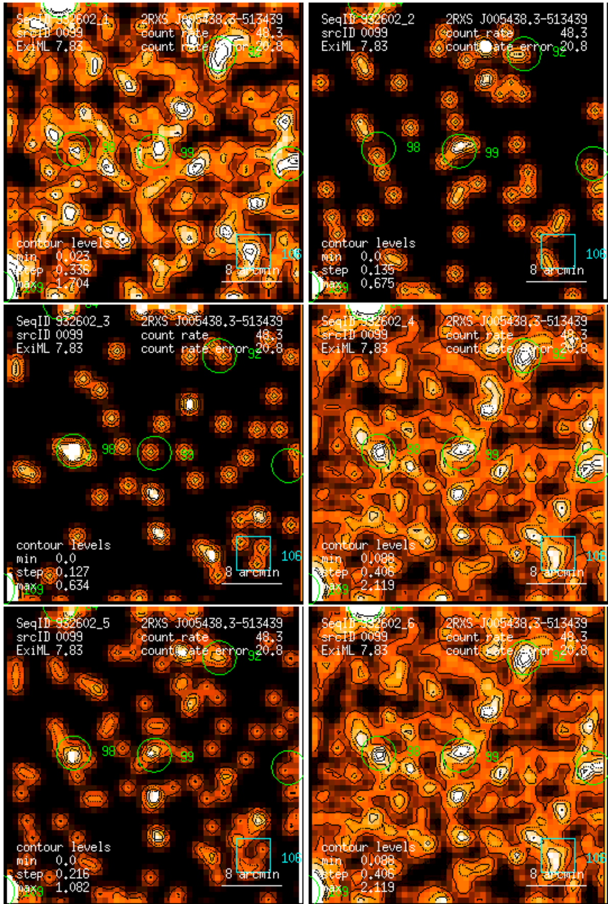
Figure 99: RASS 932602: detection 0099: band rate images, Gaussian filter: (1) PSPC channels 11 – 41, (2) 52 – 90, (3) 91 – 201, (4) 11 – 235, (5) 52 – 201, (6) 11 – 201. Broad band rates in counts/ks. Band rate contour levels in counts/ks/arcmin 2 .
