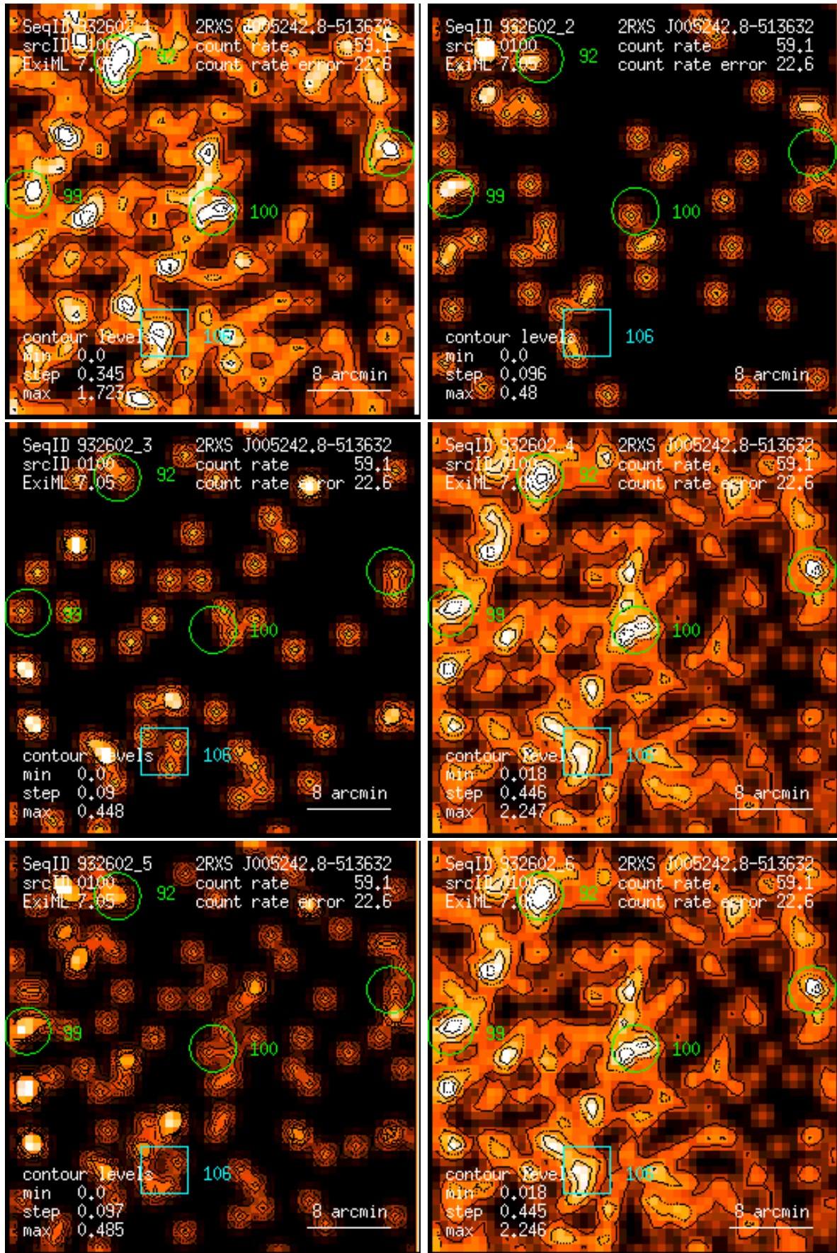
Figure 100: RASS 932602: detection 0100: band rate images, Gaussian filter: (1) PSPC channels 11 – 41, (2) 52 – 90, (3) 91 – 201, (4) 11 – 235, (5) 52 – 201, (6) 11 – 201. Broad band rates in counts/ks. Band rate contour levels in counts/ks/arcmin 2 .
