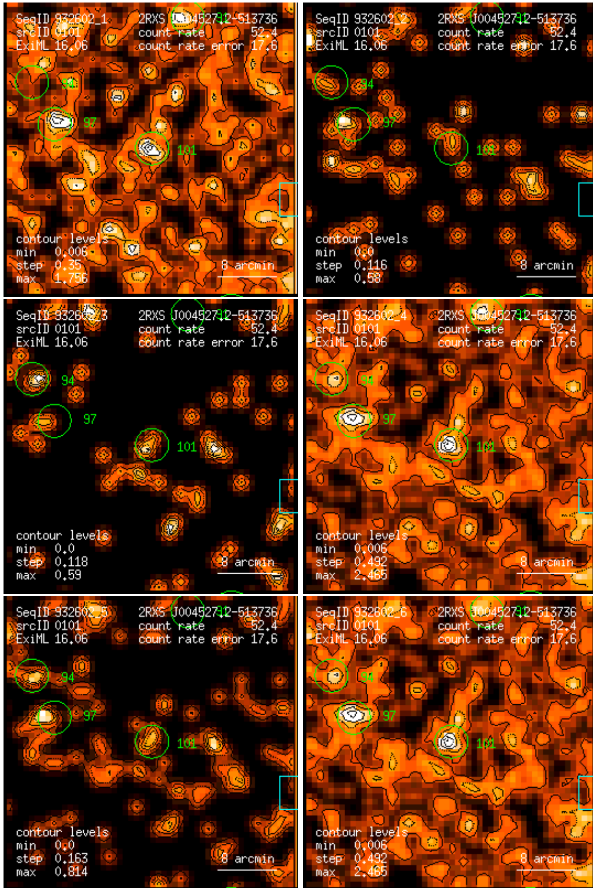
Figure 101: RASS 932602: detection 0101: band rate images, Gaussian filter: (1) PSPC channels 11 – 41, (2) 52 – 90, (3) 91 – 201, (4) 11 – 235, (5) 52 – 201, (6) 11 – 201. Broad band rates in counts/ks. Band rate contour levels in counts/ks/arcmin 2 .
