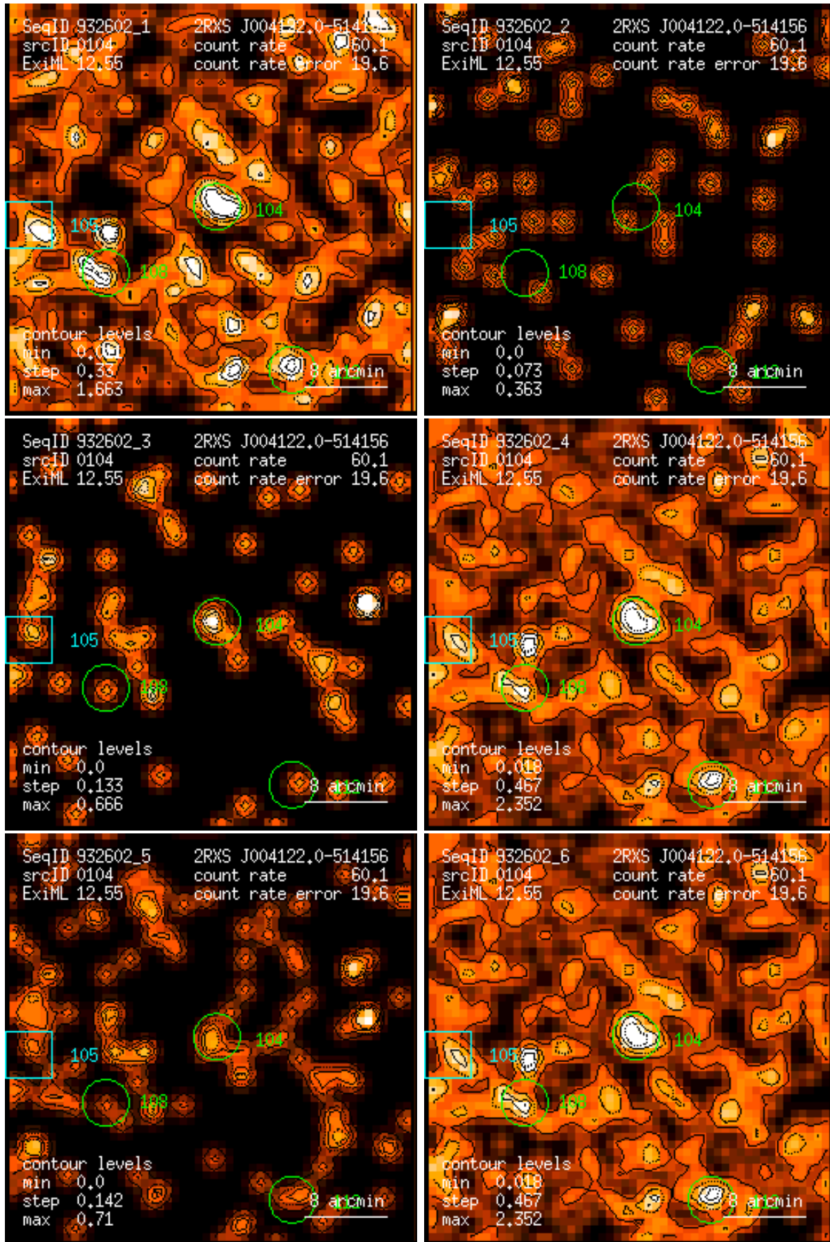
Figure 104: RASS 932602: detection 0104: band rate images, Gaussian filter: (1) PSPC channels 11 – 41, (2) 52 – 90, (3) 91 – 201, (4) 11 – 235, (5) 52 – 201, (6) 11 – 201. Broad band rates in counts/ks. Band rate contour levels in counts/ks/arcmin 2 .
