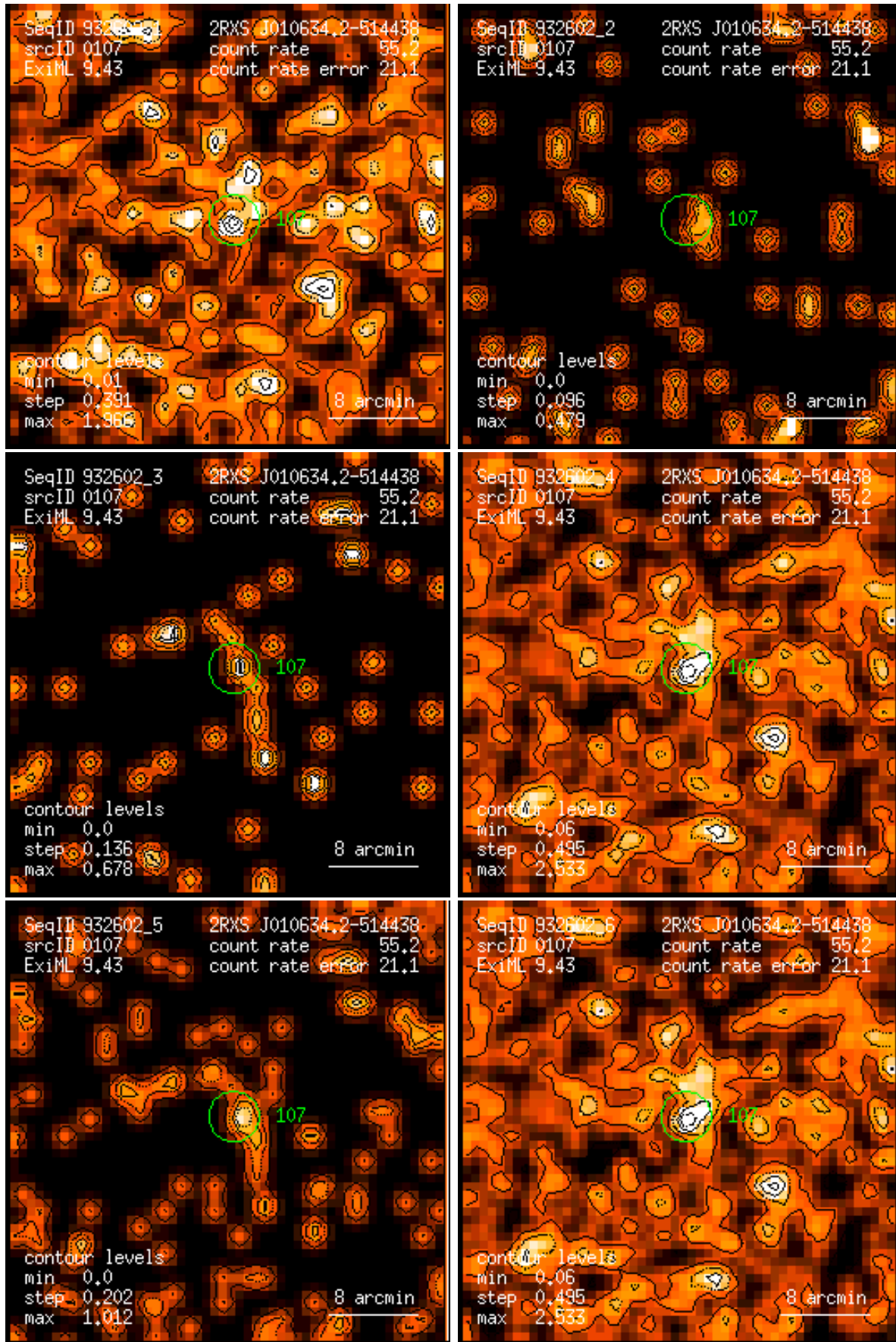
Figure 107: RASS 932602: detection 0107: band rate images, Gaussian filter: (1) PSPC channels 11 – 41, (2) 52 – 90, (3) 91 – 201, (4) 11 – 235, (5) 52 – 201, (6) 11 – 201. Broad band rates in counts/ks. Band rate contour levels in counts/ks/arcmin 2 .
