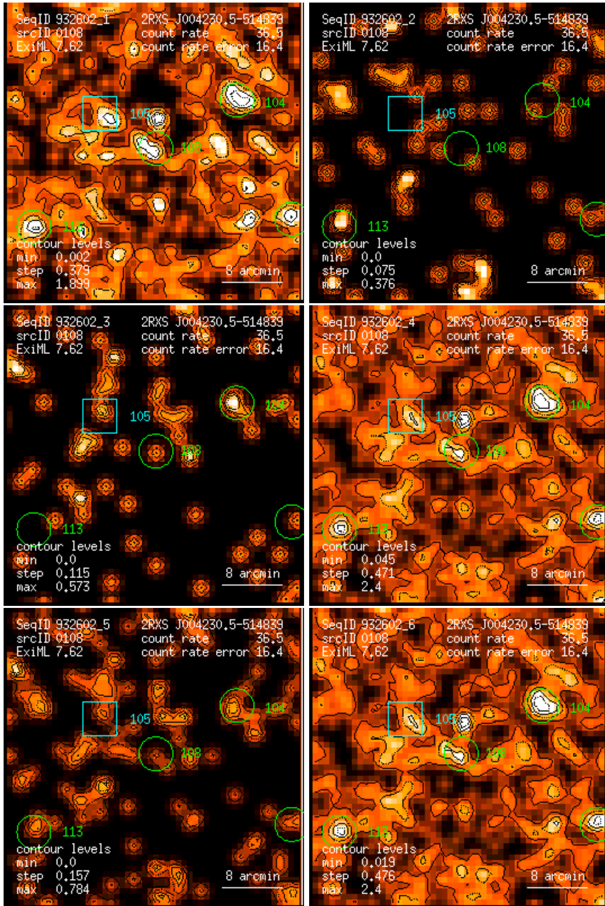
Figure 108: RASS 932602: detection 0108: band rate images, Gaussian filter: (1) PSPC channels 11 – 41, (2) 52 – 90, (3) 91 – 201, (4) 11 – 235, (5) 52 – 201, (6) 11 – 201. Broad band rates in counts/ks. Band rate contour levels in counts/ks/arcmin 2 .
