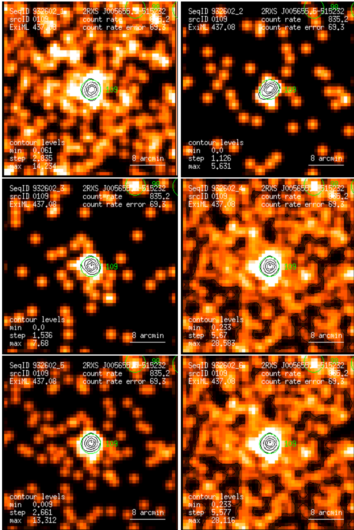
Figure 109: RASS 932602: detection 0109: band rate images, Gaussian filter: (1) PSPC channels 11 – 41, (2) 52 – 90, (3) 91 – 201, (4) 11 – 235, (5) 52 – 201, (6) 11 – 201. Broad band rates in counts/ks. Band rate contour levels in counts/ks/arcmin 2 .
