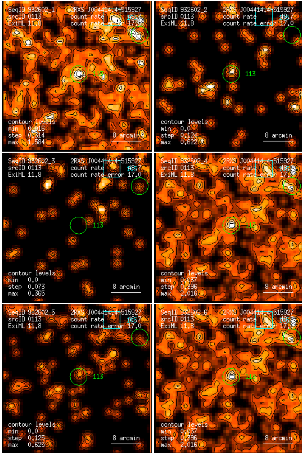
Figure 113: RASS 932602: detection 0113: band rate images, Gaussian filter: (1) PSPC channels 11 – 41, (2) 52 – 90, (3) 91 – 201, (4) 11 – 235, (5) 52 – 201, (6) 11 – 201. Broad band rates in counts/ks. Band rate contour levels in counts/ks/arcmin 2 .
