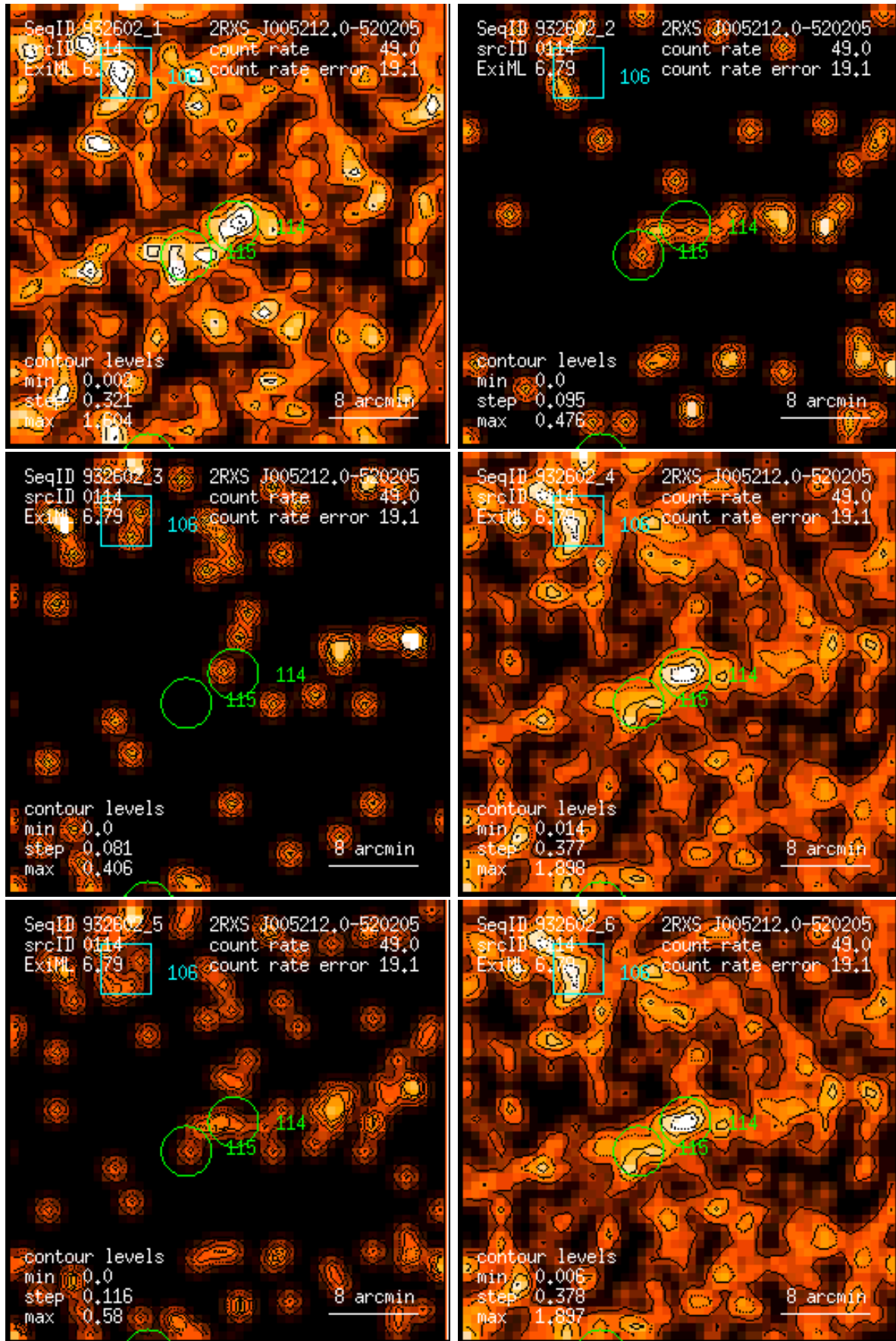
Figure 114: RASS 932602: detection 0114: band rate images, Gaussian filter: (1) PSPC channels 11 – 41, (2) 52 – 90, (3) 91 – 201, (4) 11 – 235, (5) 52 – 201, (6) 11 – 201. Broad band rates in counts/ks. Band rate contour levels in counts/ks/arcmin 2 .
