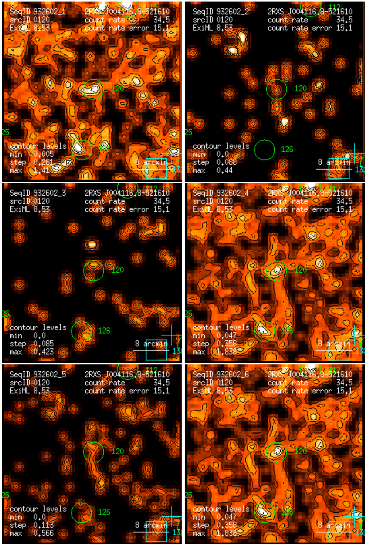
Figure 120: RASS 932602: detection 0120: band rate images, Gaussian filter: (1) PSPC channels 11 – 41, (2) 52 – 90, (3) 91 – 201, (4) 11 – 235, (5) 52 – 201, (6) 11 – 201. Broad band rates in counts/ks. Band rate contour levels in counts/ks/arcmin 2 .
