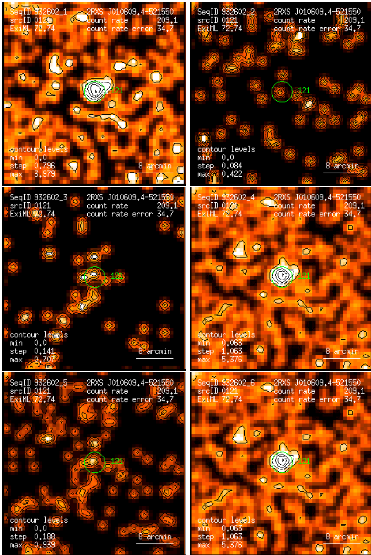
Figure 121: RASS 932602: detection 0121: band rate images, Gaussian filter: (1) PSPC channels 11 – 41, (2) 52 – 90, (3) 91 – 201, (4) 11 – 235, (5) 52 – 201, (6) 11 – 201. Broad band rates in counts/ks. Band rate contour levels in counts/ks/arcmin 2 .
