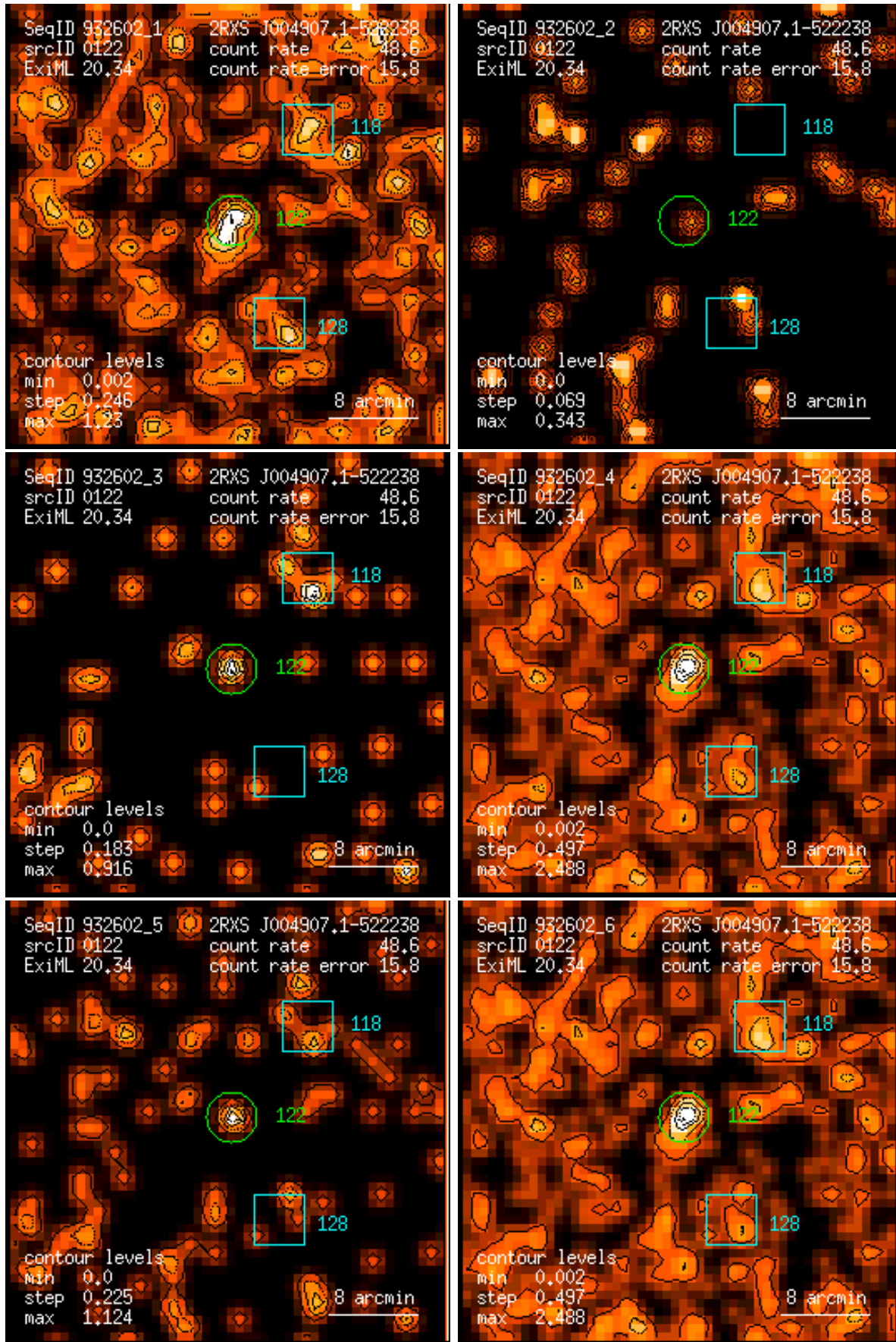
Figure 122: RASS 932602: detection 0122: band rate images, Gaussian filter: (1) PSPC channels 11 – 41, (2) 52 – 90, (3) 91 – 201, (4) 11 – 235, (5) 52 – 201, (6) 11 – 201. Broad band rates in counts/ks. Band rate contour levels in counts/ks/arcmin 2 .
