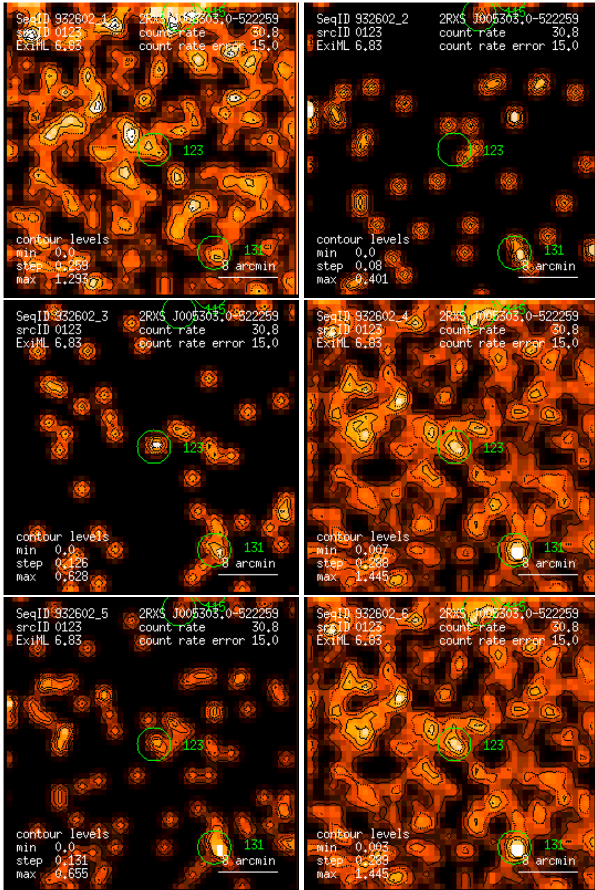
Figure 123: RASS 932602: detection 0123: band rate images, Gaussian filter: (1) PSPC channels 11 – 41, (2) 52 – 90, (3) 91 – 201, (4) 11 – 235, (5) 52 – 201, (6) 11 – 201. Broad band rates in counts/ks. Band rate contour levels in counts/ks/arcmin 2 .
