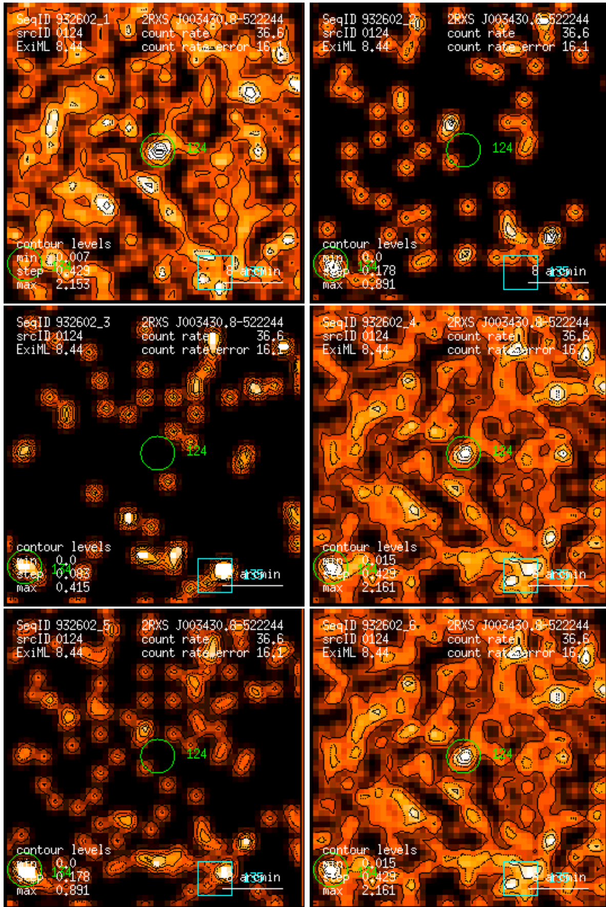
Figure 124: RASS 932602: detection 0124: band rate images, Gaussian filter: (1) PSPC channels 11 – 41, (2) 52 – 90, (3) 91 – 201, (4) 11 – 235, (5) 52 – 201, (6) 11 – 201. Broad band rates in counts/ks. Band rate contour levels in counts/ks/arcmin 2 .
