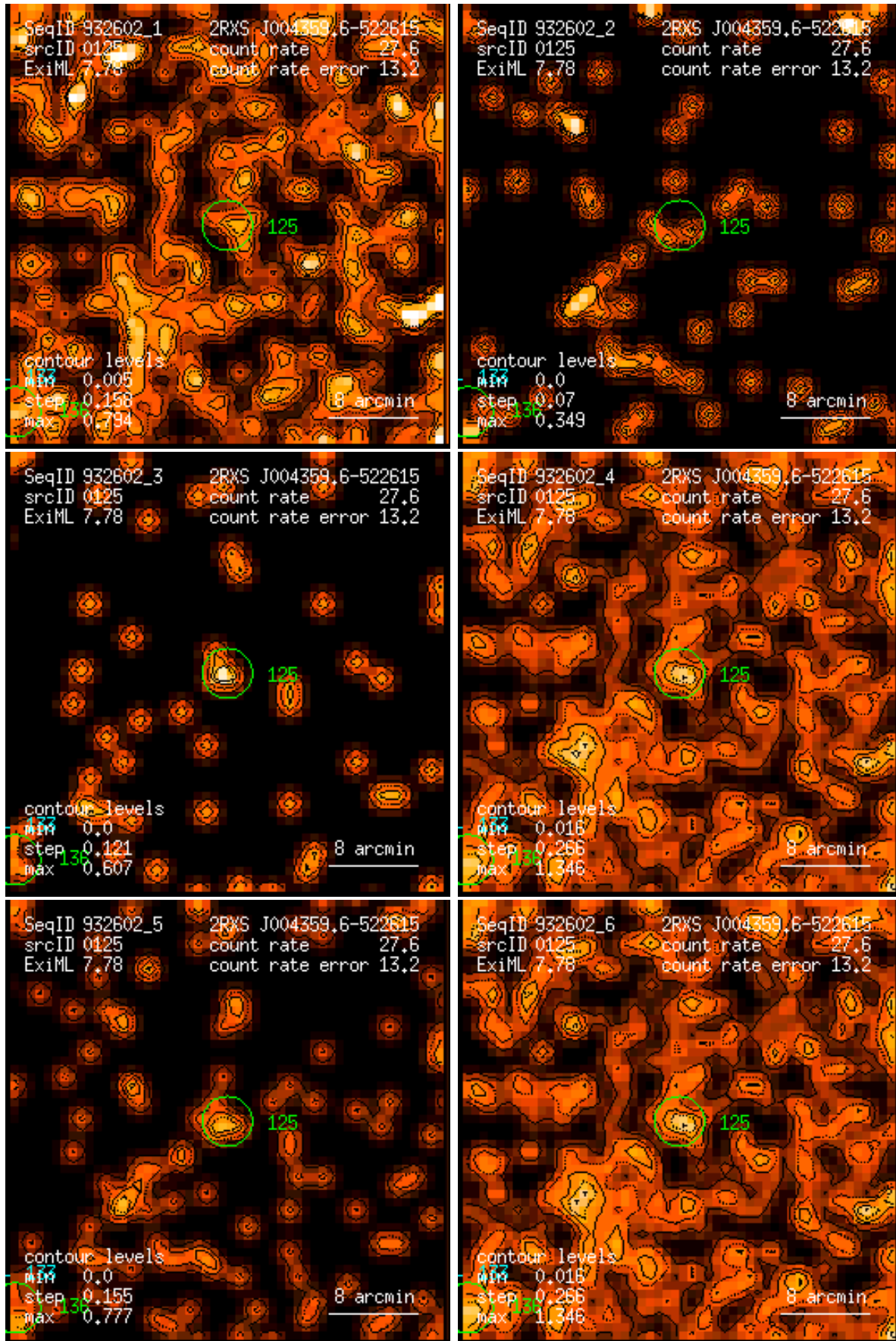
Figure 125: RASS 932602: detection 0125: band rate images, Gaussian filter: (1) PSPC channels 11 – 41, (2) 52 – 90, (3) 91 – 201, (4) 11 – 235, (5) 52 – 201, (6) 11 – 201. Broad band rates in counts/ks. Band rate contour levels in counts/ks/arcmin 2 .
