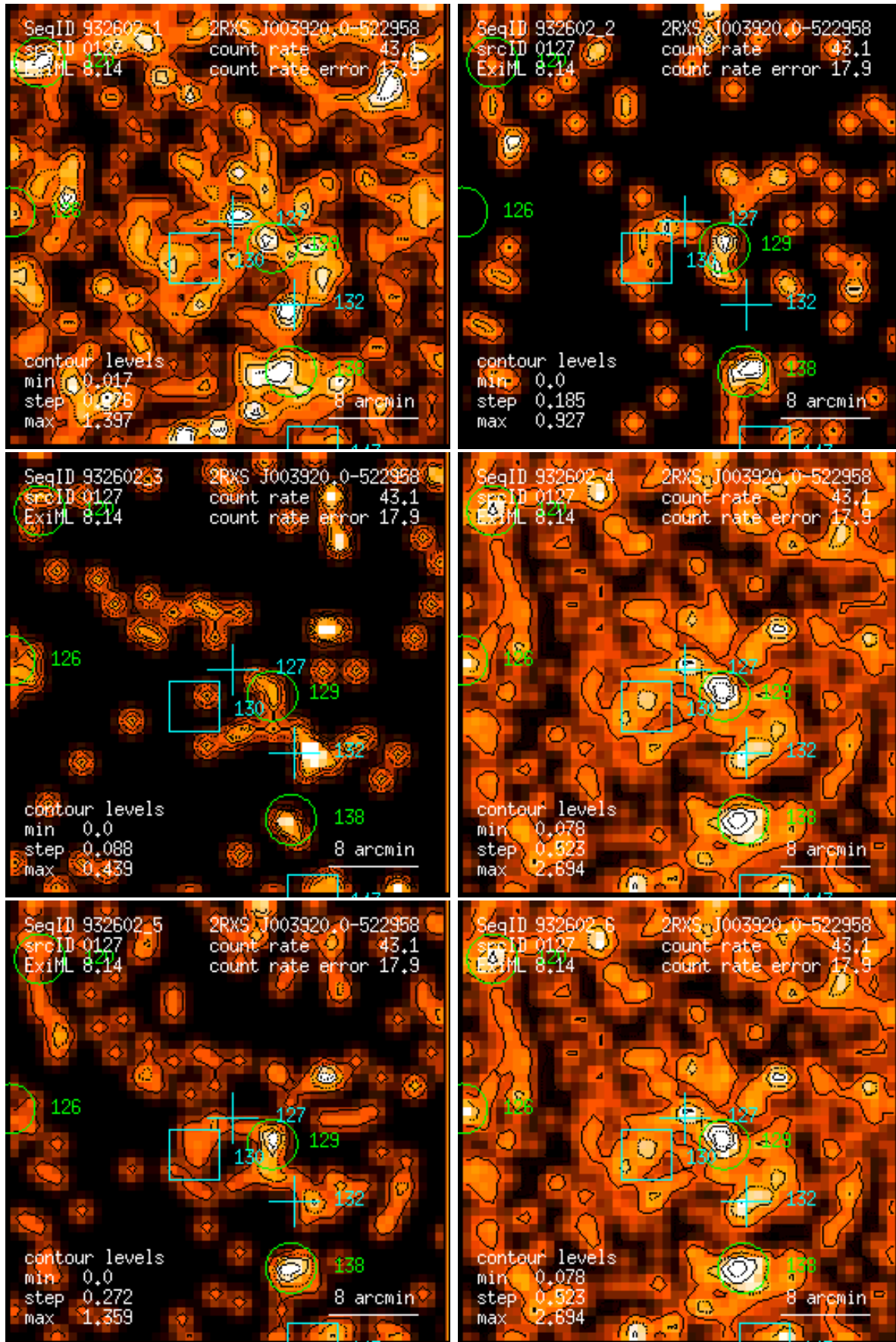
Figure 127: RASS 932602: detection 0127: band rate images, Gaussian filter: (1) PSPC channels 11 – 41, (2) 52 – 90, (3) 91 – 201, (4) 11 – 235, (5) 52 – 201, (6) 11 – 201. Broad band rates in counts/ks. Band rate contour levels in counts/ks/arcmin 2 .
