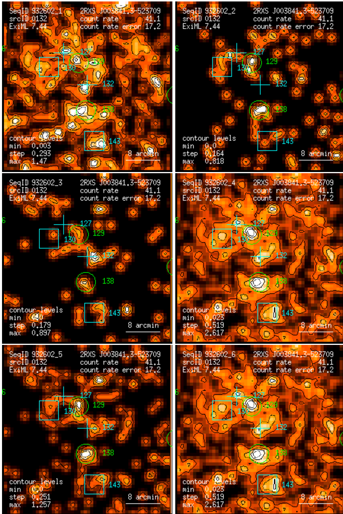
Figure 132: RASS 932602: detection 0132: band rate images, Gaussian filter: (1) PSPC channels 11 – 41, (2) 52 – 90, (3) 91 – 201, (4) 11 – 235, (5) 52 – 201, (6) 11 – 201. Broad band rates in counts/ks. Band rate contour levels in counts/ks/arcmin 2 .
