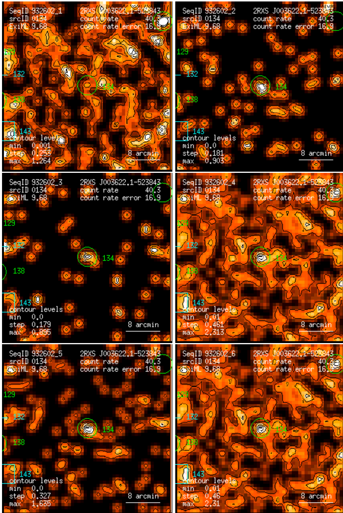
Figure 134: RASS 932602: detection 0134: band rate images, Gaussian filter: (1) PSPC channels 11 – 41, (2) 52 – 90, (3) 91 – 201, (4) 11 – 235, (5) 52 – 201, (6) 11 – 201. Broad band rates in counts/ks. Band rate contour levels in counts/ks/arcmin 2 .
