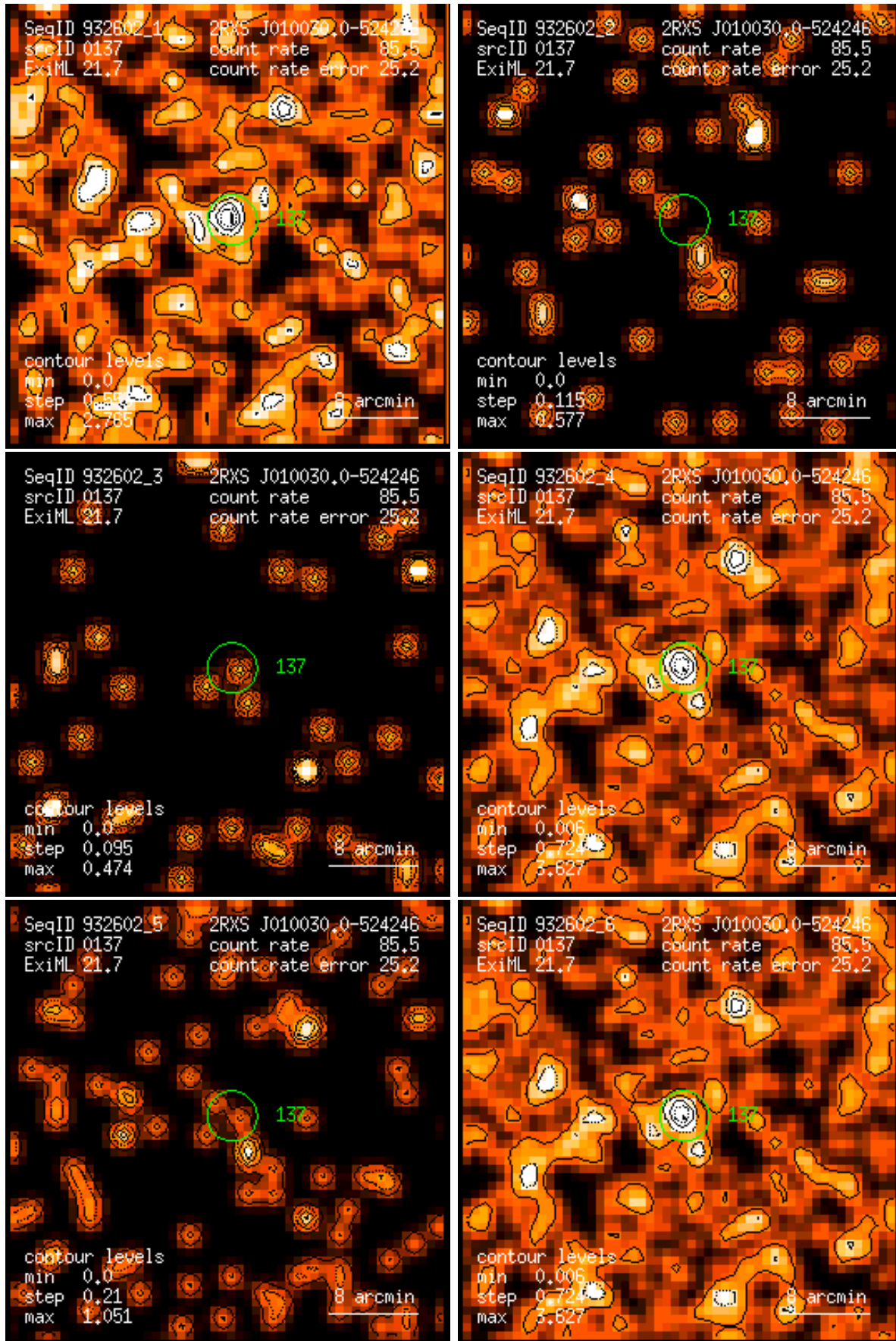
Figure 137: RASS 932602: detection 0137: band rate images, Gaussian filter: (1) PSPC channels 11 – 41, (2) 52 – 90, (3) 91 – 201, (4) 11 – 235, (5) 52 – 201, (6) 11 – 201. Broad band rates in counts/ks. Band rate contour levels in counts/ks/arcmin 2 .
