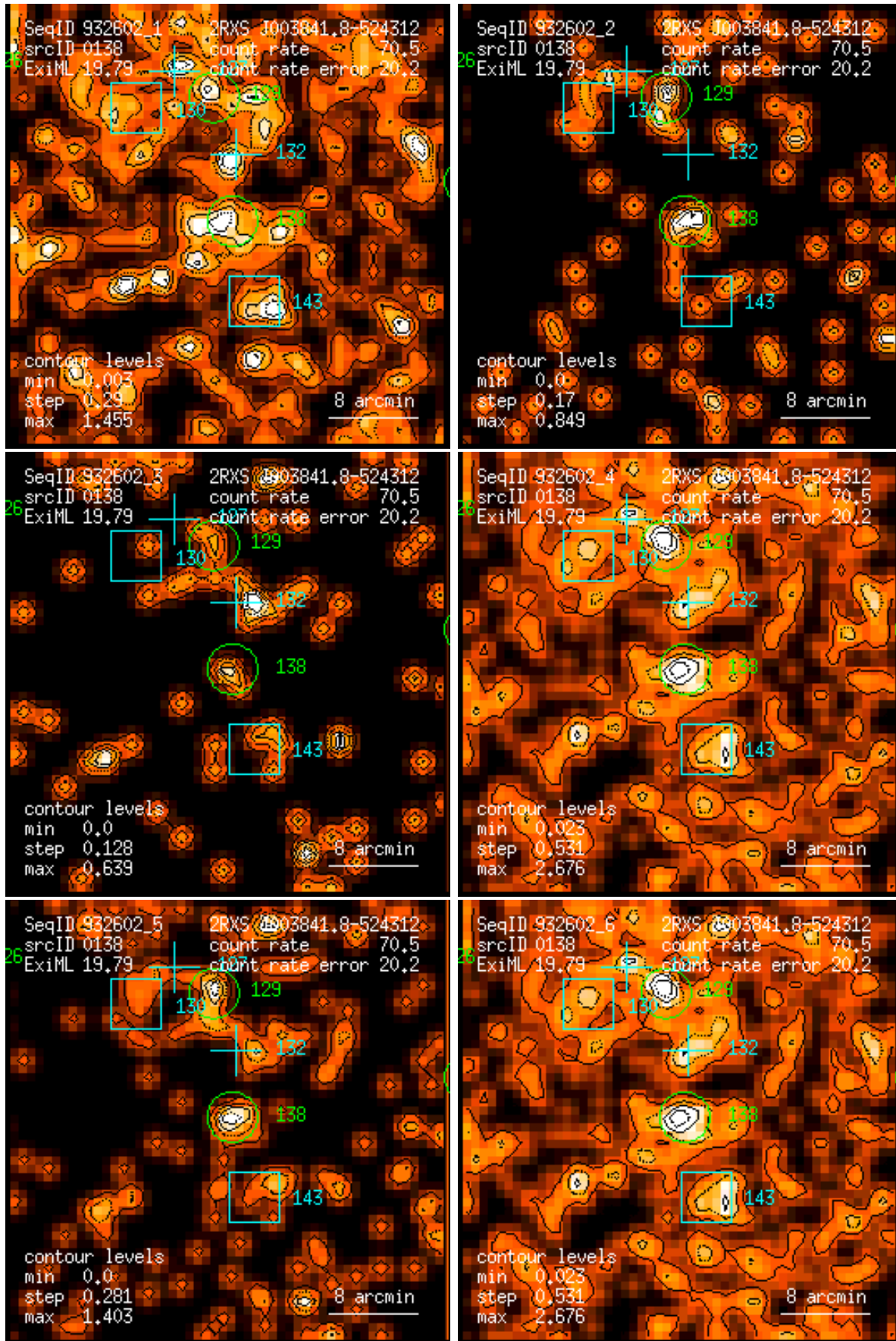
Figure 138: RASS 932602: detection 0138: band rate images, Gaussian filter: (1) PSPC channels 11 – 41, (2) 52 – 90, (3) 91 – 201, (4) 11 – 235, (5) 52 – 201, (6) 11 – 201. Broad band rates in counts/ks. Band rate contour levels in counts/ks/arcmin 2 .
