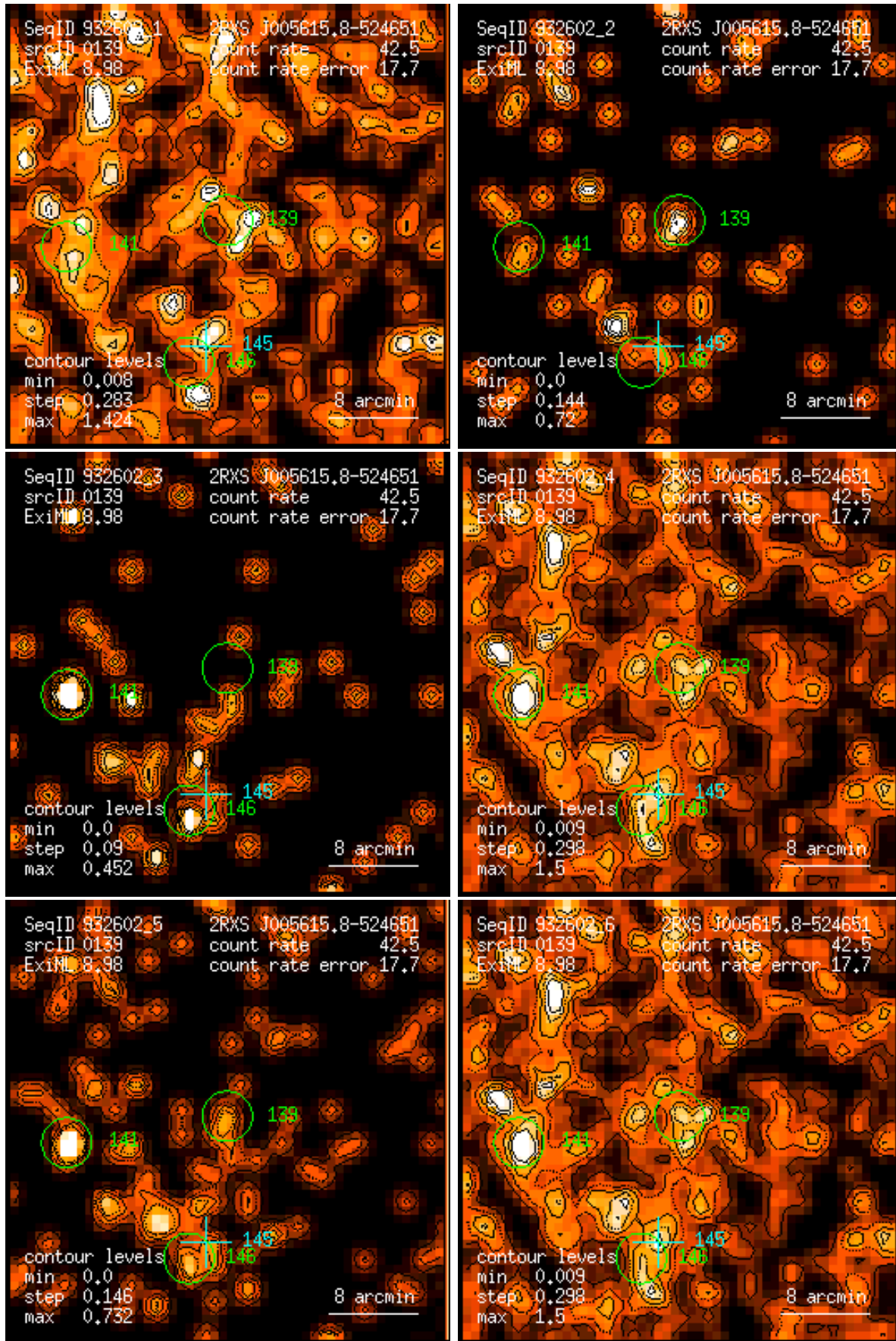
Figure 139: RASS 932602: detection 0139: band rate images, Gaussian filter: (1) PSPC channels 11 – 41, (2) 52 – 90, (3) 91 – 201, (4) 11 – 235, (5) 52 – 201, (6) 11 – 201. Broad band rates in counts/ks. Band rate contour levels in counts/ks/arcmin 2 .
