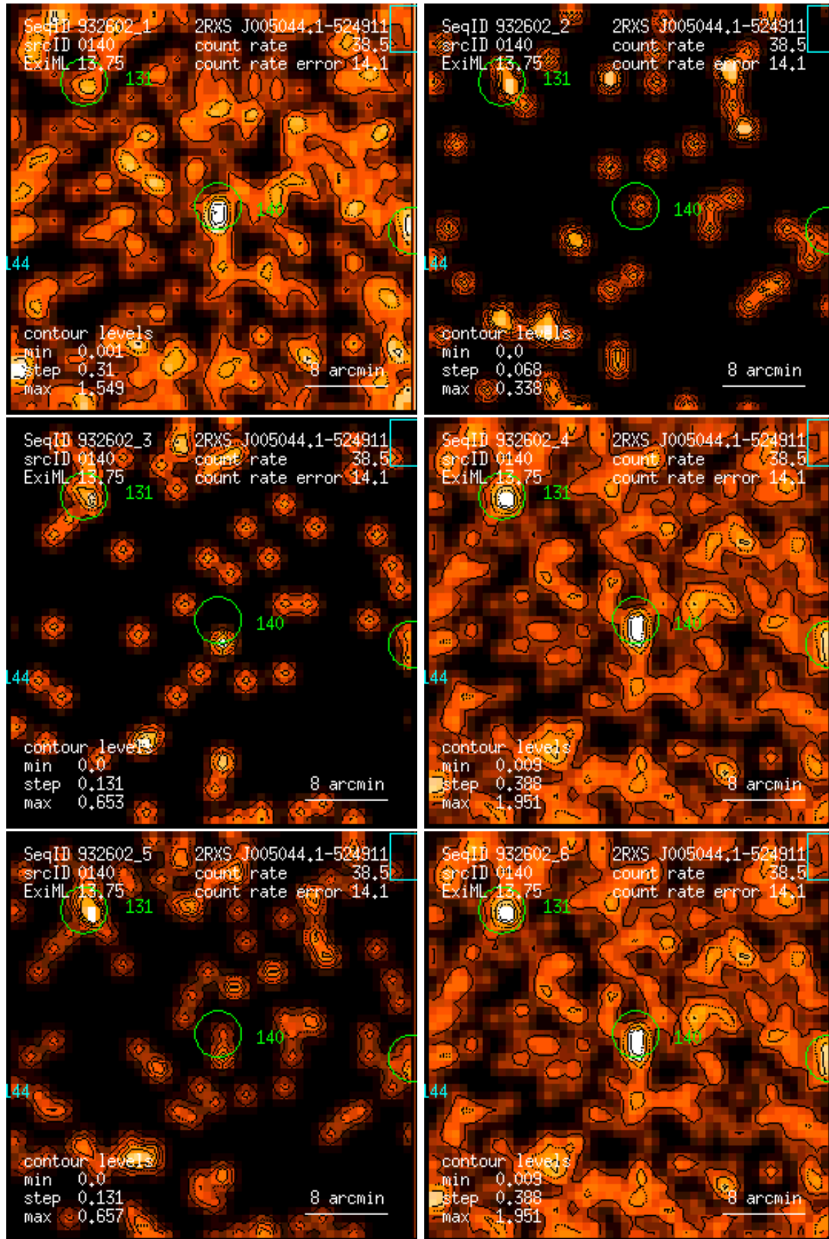
Figure 140: RASS 932602: detection 0140: band rate images, Gaussian filter: (1) PSPC channels 11 – 41, (2) 52 – 90, (3) 91 – 201, (4) 11 – 235, (5) 52 – 201, (6) 11 – 201. Broad band rates in counts/ks. Band rate contour levels in counts/ks/arcmin 2 .
