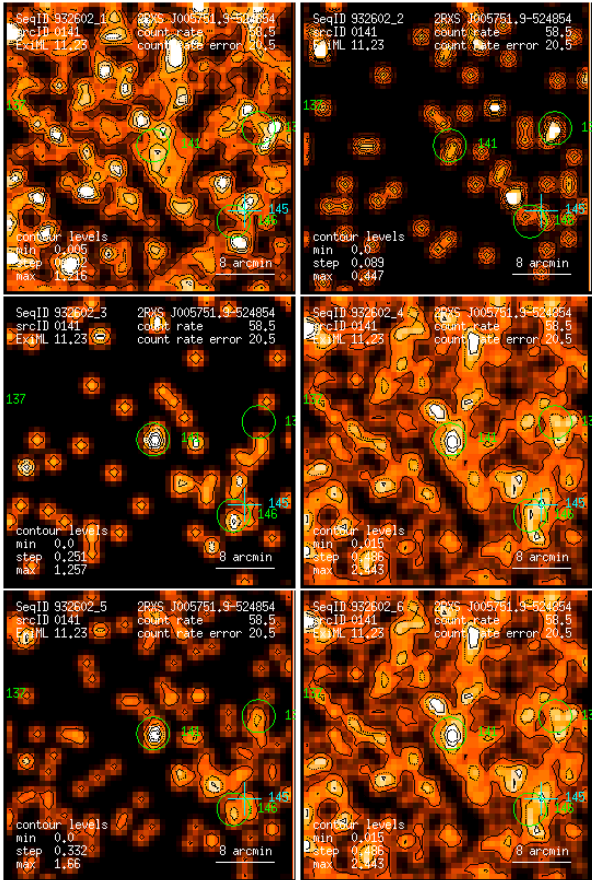
Figure 141: RASS 932602: detection 0141: band rate images, Gaussian filter: (1) PSPC channels 11 – 41, (2) 52 – 90, (3) 91 – 201, (4) 11 – 235, (5) 52 – 201, (6) 11 – 201. Broad band rates in counts/ks. Band rate contour levels in counts/ks/arcmin 2 .
