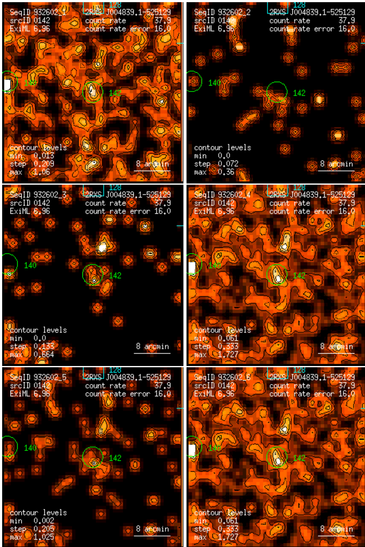
Figure 142: RASS 932602: detection 0142: band rate images, Gaussian filter: (1) PSPC channels 11 – 41, (2) 52 – 90, (3) 91 – 201, (4) 11 – 235, (5) 52 – 201, (6) 11 – 201. Broad band rates in counts/ks. Band rate contour levels in counts/ks/arcmin 2 .
