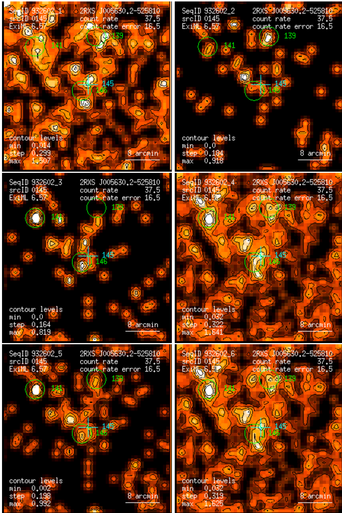
Figure 145: RASS 932602: detection 0145: band rate images, Gaussian filter: (1) PSPC channels 11 – 41, (2) 52 – 90, (3) 91 – 201, (4) 11 – 235, (5) 52 – 201, (6) 11 – 201. Broad band rates in counts/ks. Band rate contour levels in counts/ks/arcmin 2 .
