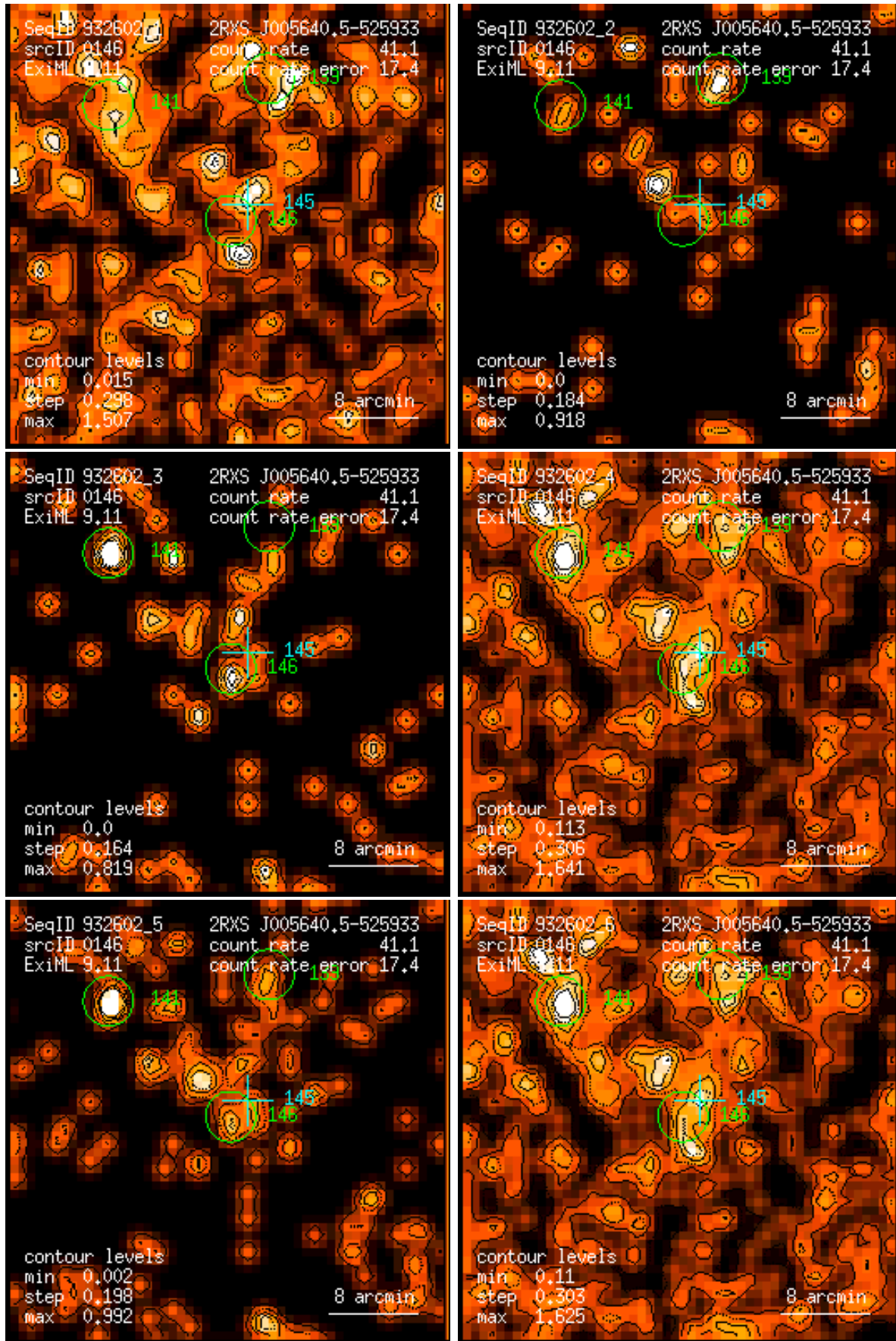
Figure 146: RASS 932602: detection 0146: band rate images, Gaussian filter: (1) PSPC channels 11 – 41, (2) 52 – 90, (3) 91 – 201, (4) 11 – 235, (5) 52 – 201, (6) 11 – 201. Broad band rates in counts/ks. Band rate contour levels in counts/ks/arcmin 2 .
