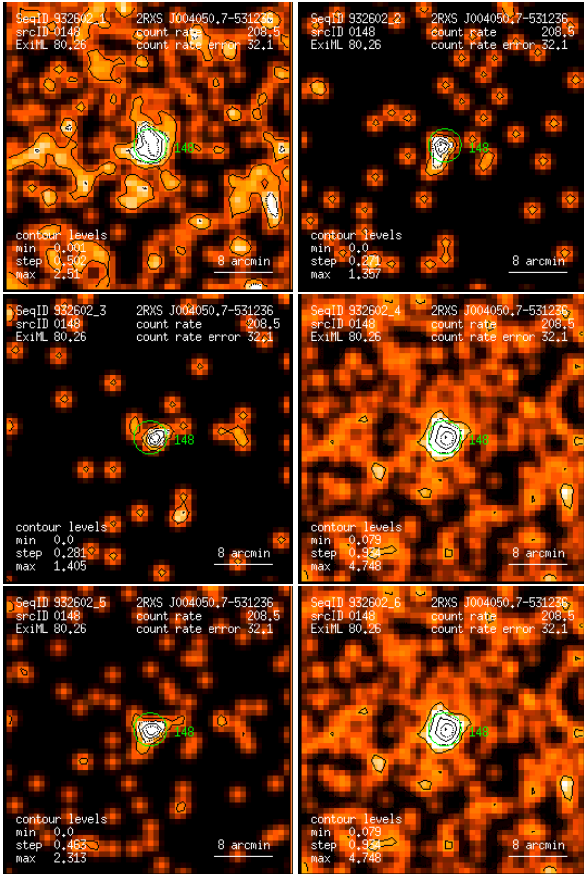
Figure 148: RASS 932602: detection 0148: band rate images, Gaussian filter: (1) PSPC channels 11 – 41, (2) 52 – 90, (3) 91 – 201, (4) 11 – 235, (5) 52 – 201, (6) 11 – 201. Broad band rates in counts/ks. Band rate contour levels in counts/ks/arcmin 2 .
