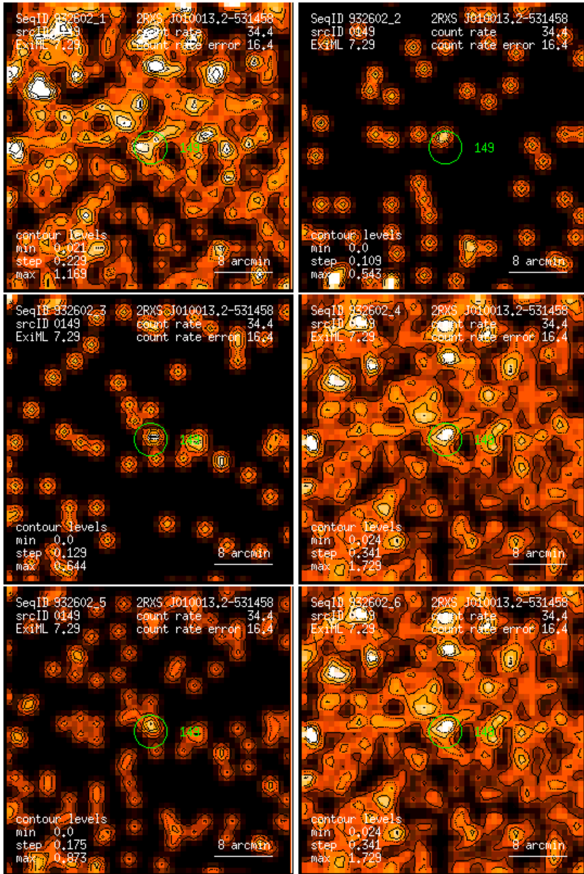
Figure 149: RASS 932602: detection 0149: band rate images, Gaussian filter: (1) PSPC channels 11 – 41, (2) 52 – 90, (3) 91 – 201, (4) 11 – 235, (5) 52 – 201, (6) 11 – 201. Broad band rates in counts/ks. Band rate contour levels in counts/ks/arcmin 2 .
